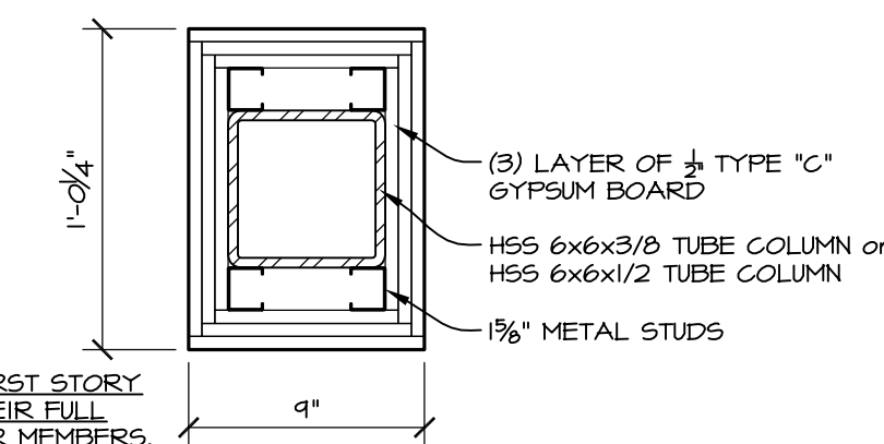
2 WRAPPED COLUMN DETAIL PC-B (3 HR.) NOT TO SCALE (IBC EQUATION 1-12)
