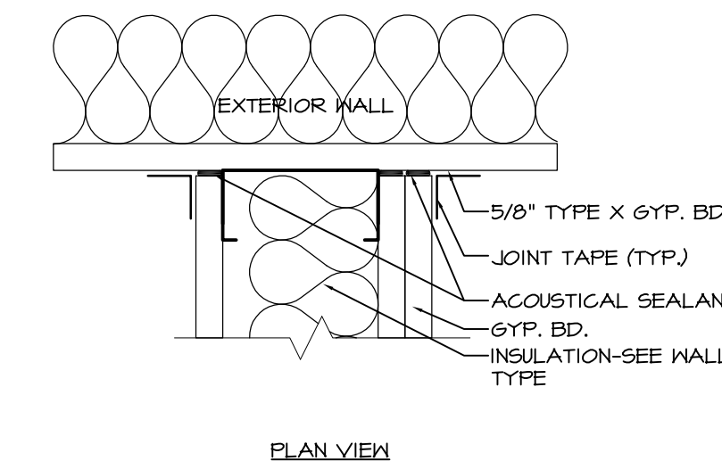
4 SOUND ISOLATION DETAIL NOT TO SCALE (TYPICAL ALL GUESTROOM AND DWELLING UNIT DEMISING WALLS)
