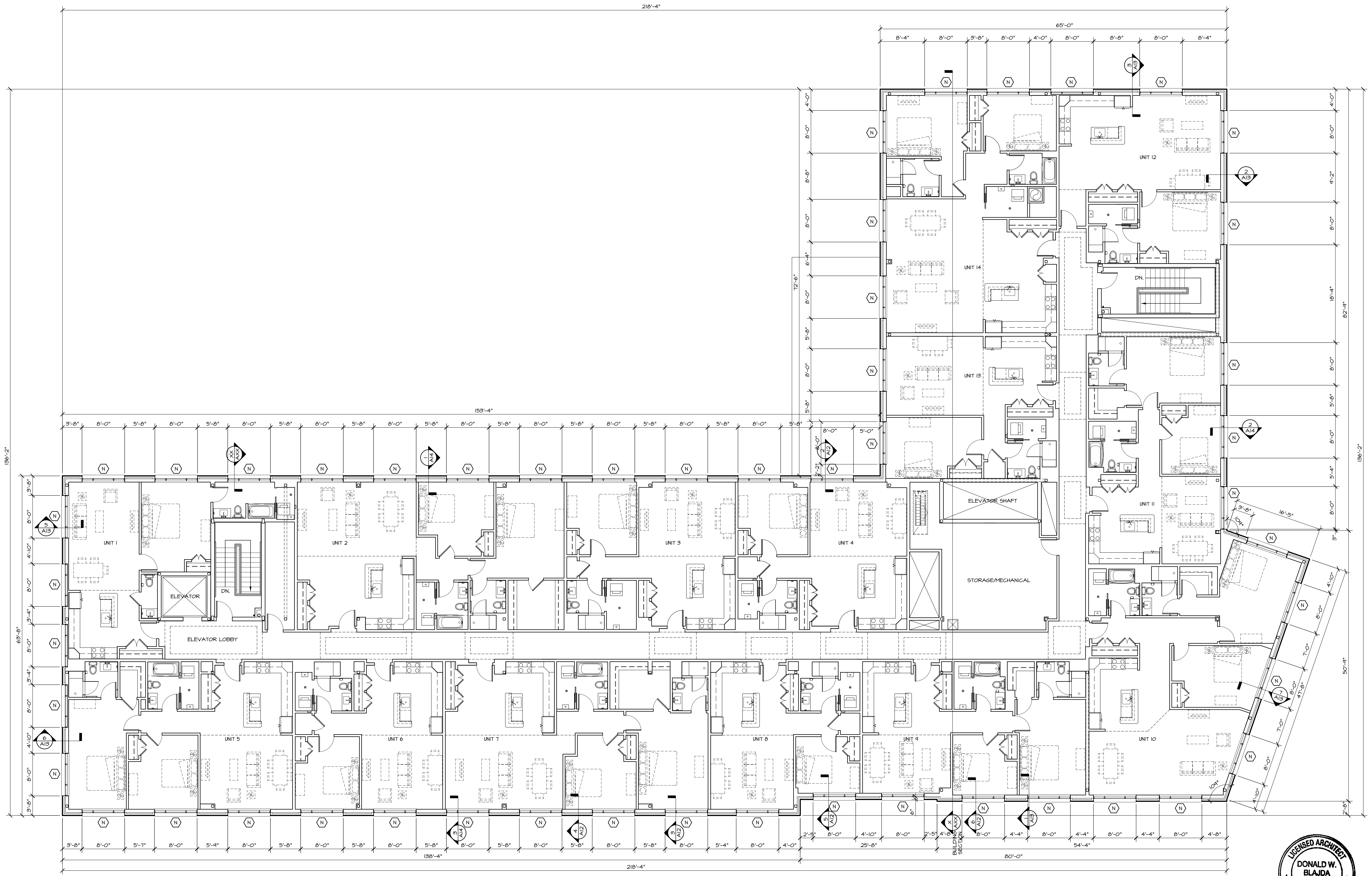
1 SIXTH FLOOR PLAN A6 1/8" = 1'-0"
