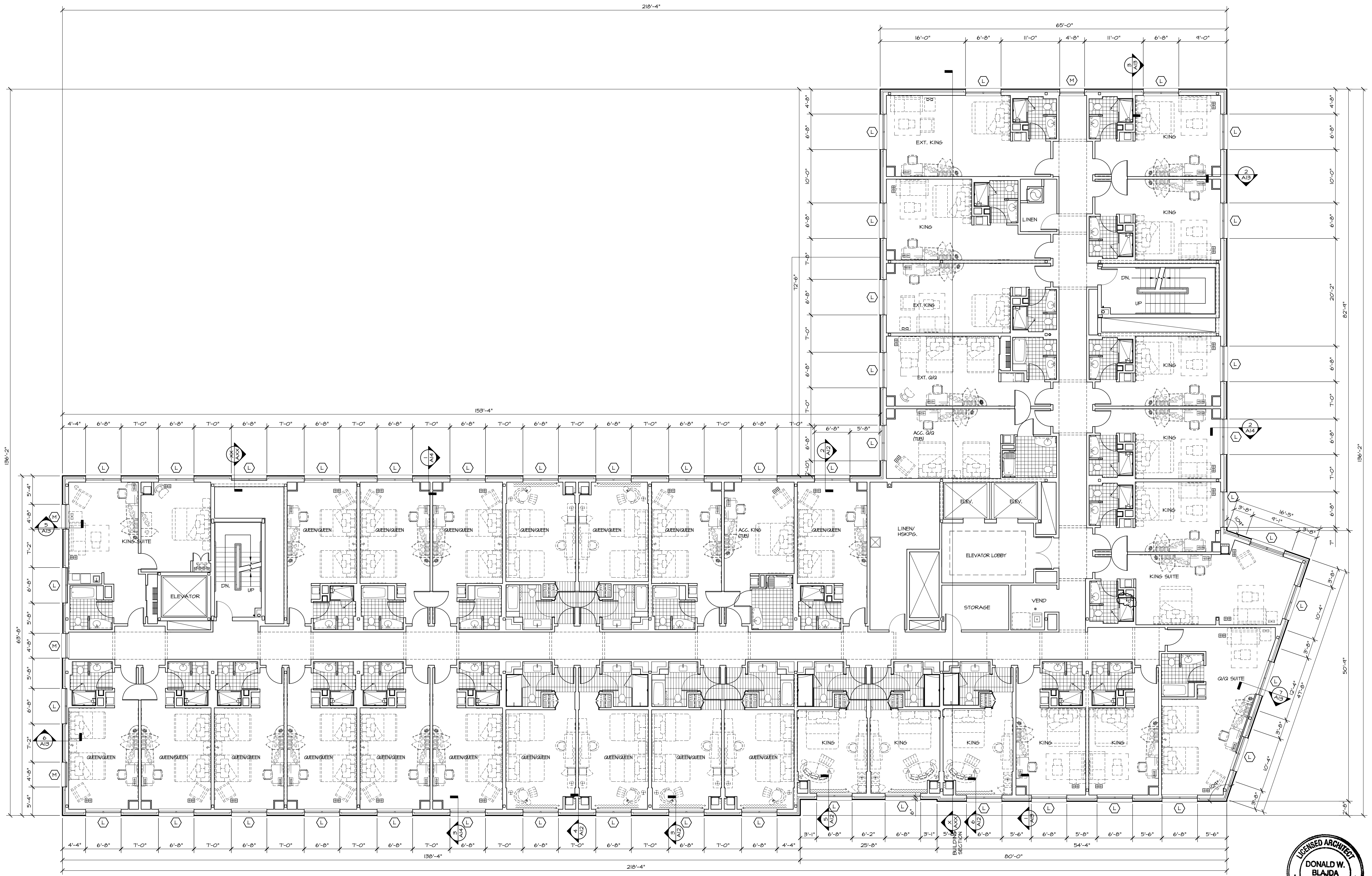
1 FOURTH FLOOR PLAN A4 1/8" = 1'-0"
