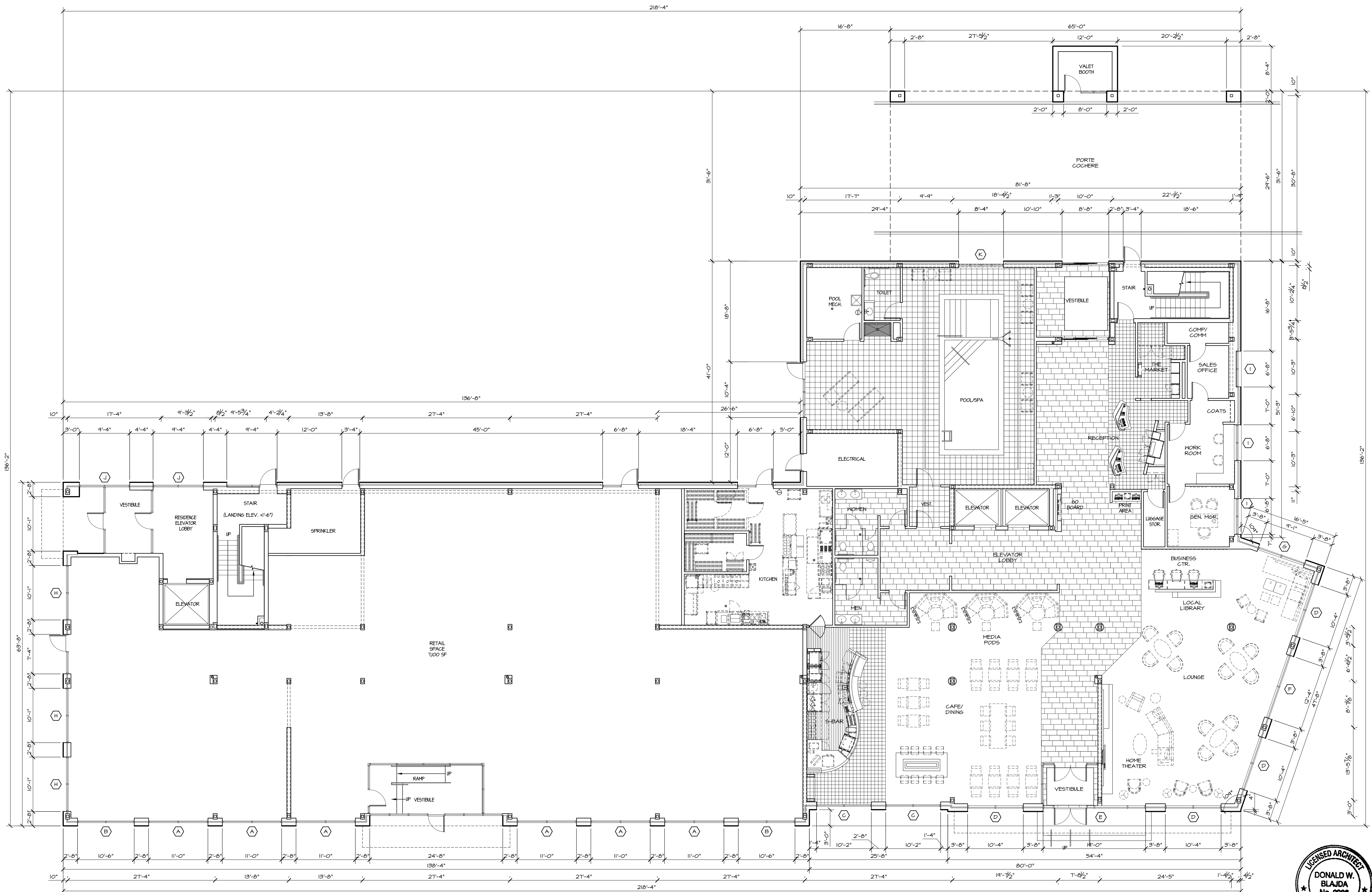
1 FIRST FLOOR PLAN A1 1/8" = 1'-0"
