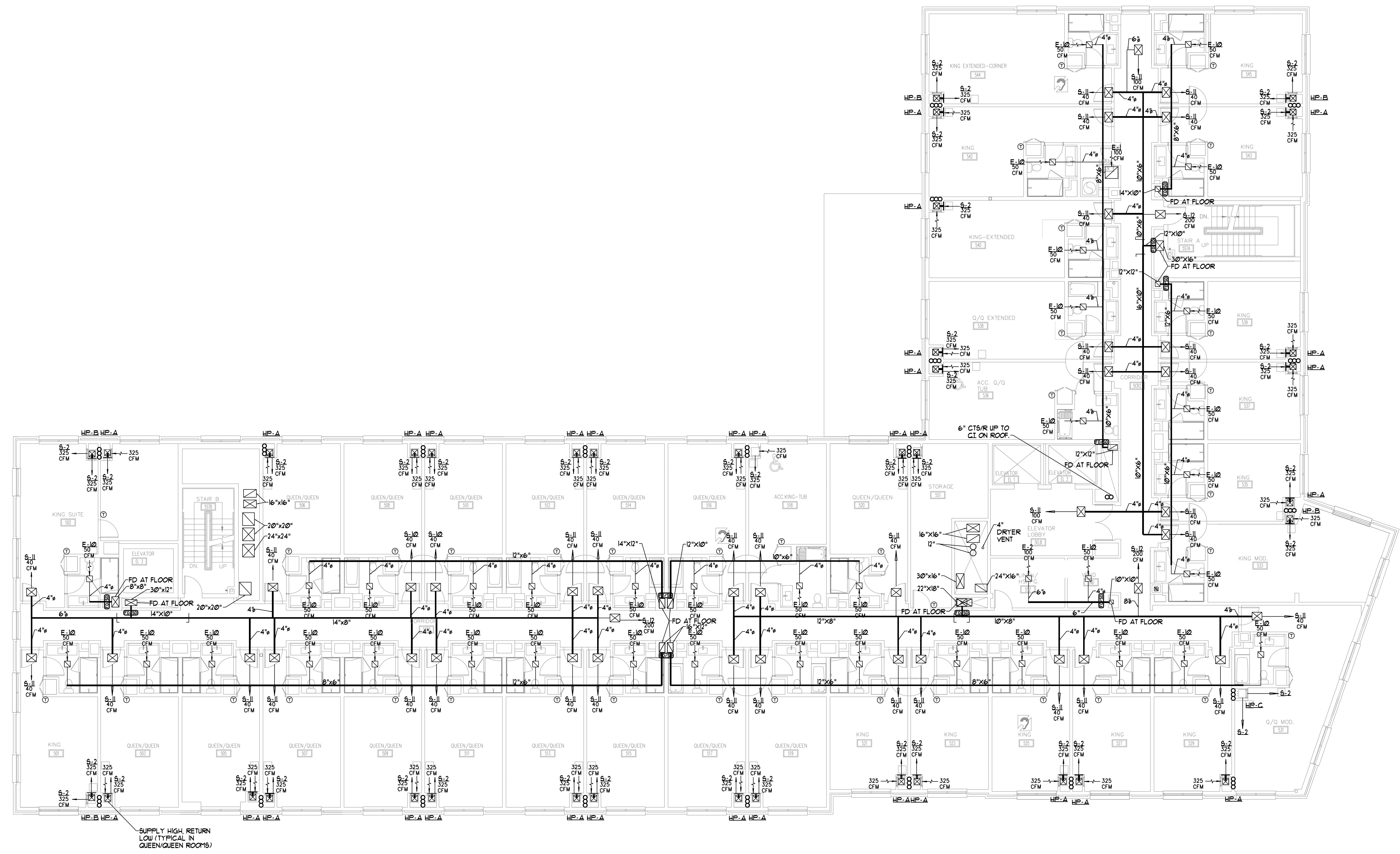
THIRD THRU FIFTH FLOOR PLAN SCALE: 1/8" = 1'-0"
