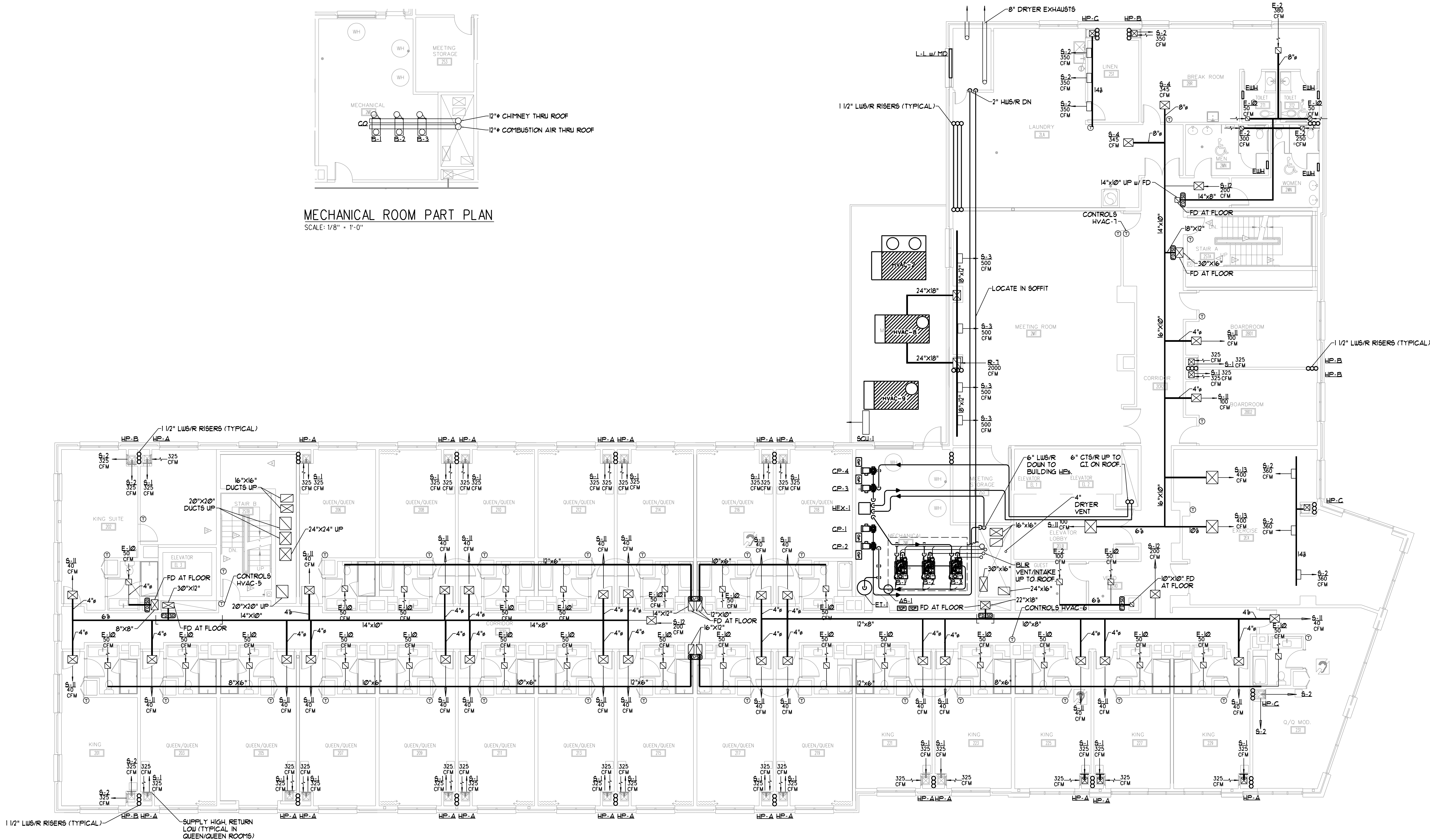
SECOND FLOOR PLAN SCALE: 1/8" = 1'-0"
