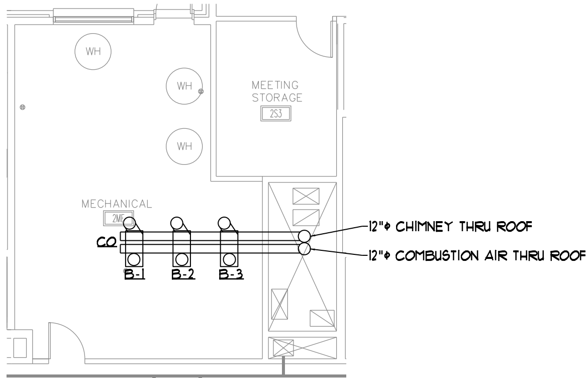
MECHANICAL ROOM PART PLAN SCALE: 1/8" = 1'-0"
