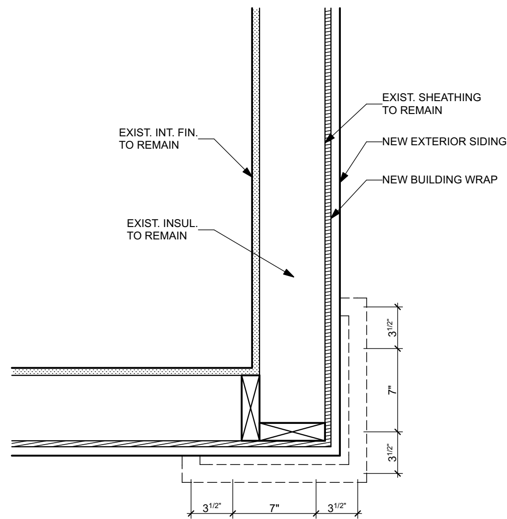
2 CORNER DETAIL SCALE: 1 1/2" = 1'-0"
