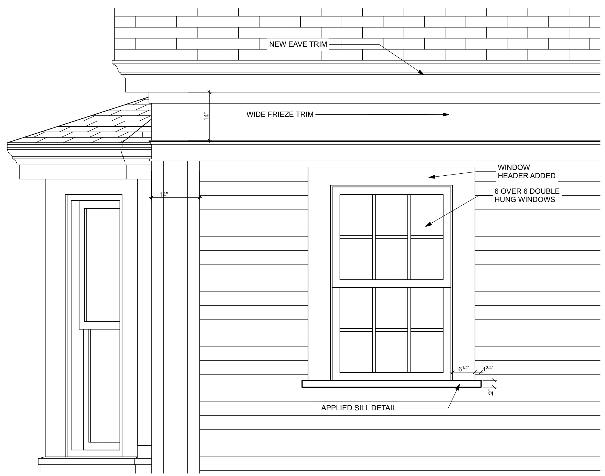
3 DETAIL - WINDOW TRIM SCALE: 3/4" = 1'-0"
