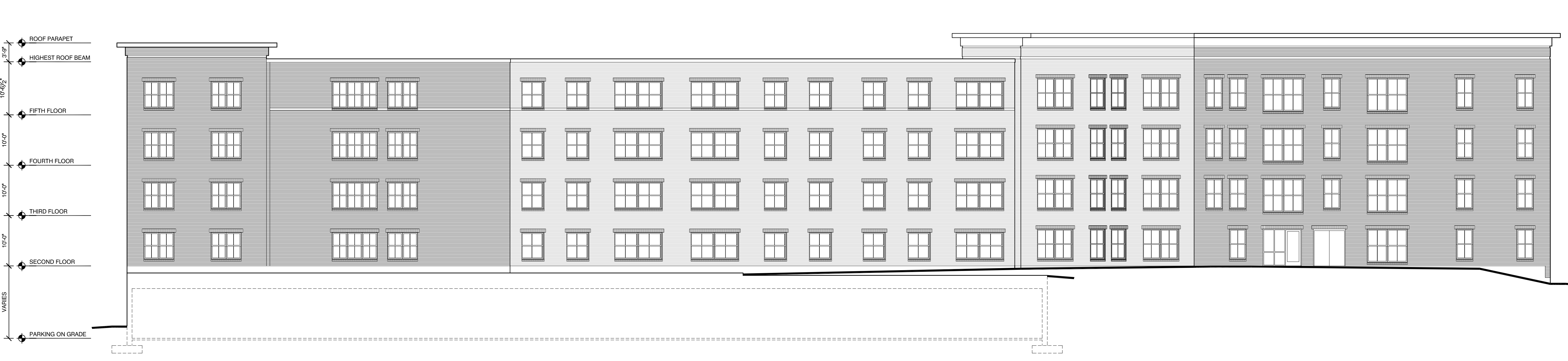
4 PARKING DECK EXTERIOR ELEVATION 3/32" = 1'-0"
