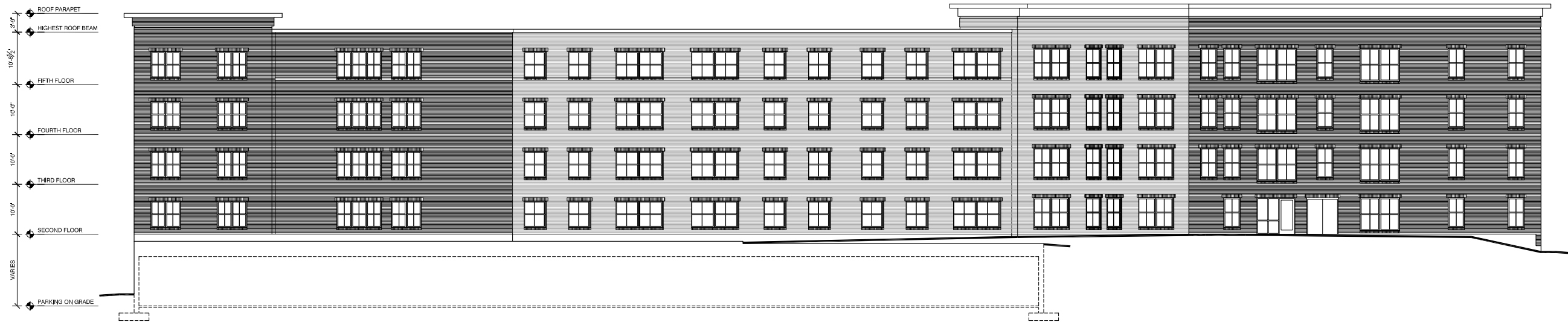
4 PARKING DECK EXTERIOR ELEVATION 3/32" = 1'-0"
