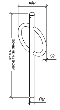
9 BIKE HITCH - ELEVATION & SECTION NOT TO SCALE
