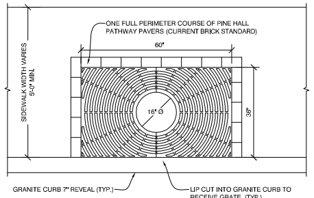
7 EXPANDABLE TREE GRATE - PLAN 1/2" = 1'-0"
