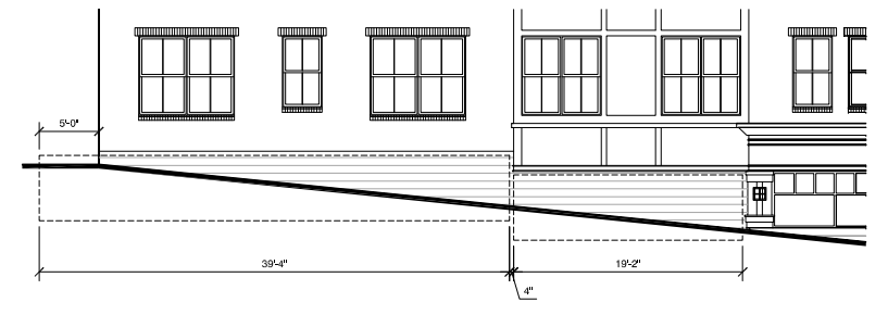
5 PLANTER - ELEVATION 1/8" = 1'-0"
