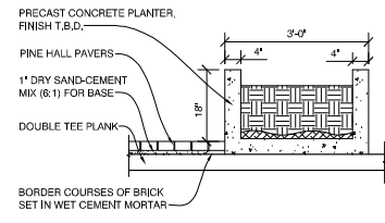
11 PATIO PLANTER - SECTION 1/2" = 1'-0"
