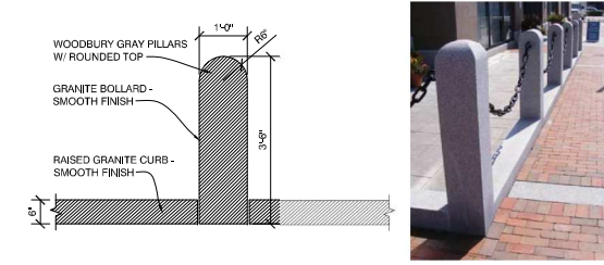
4 GRANITE BOLLARD - SECTION & EXAMPLE 1/2" = 1'-0"
