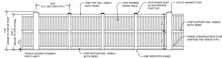
10 FENCE - ELEVATION 1/4" = 1'-0"
