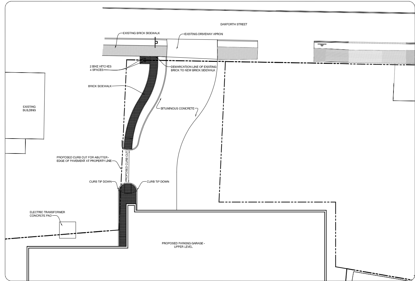
2 HARDSCAPE PLAN - PARKING GARAGE 1/16" = 1'-0"
