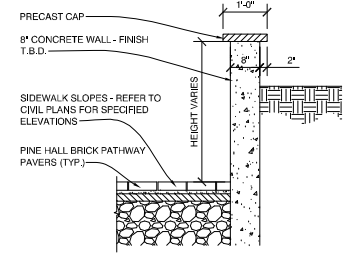
6 PLANTER - SECTION 1/2" = 1'-0"
