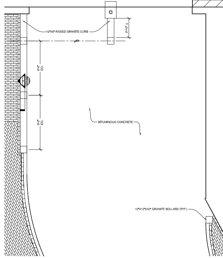
3 GRANITE BOLLARD - PLAN 1/4" = 1'-0"
