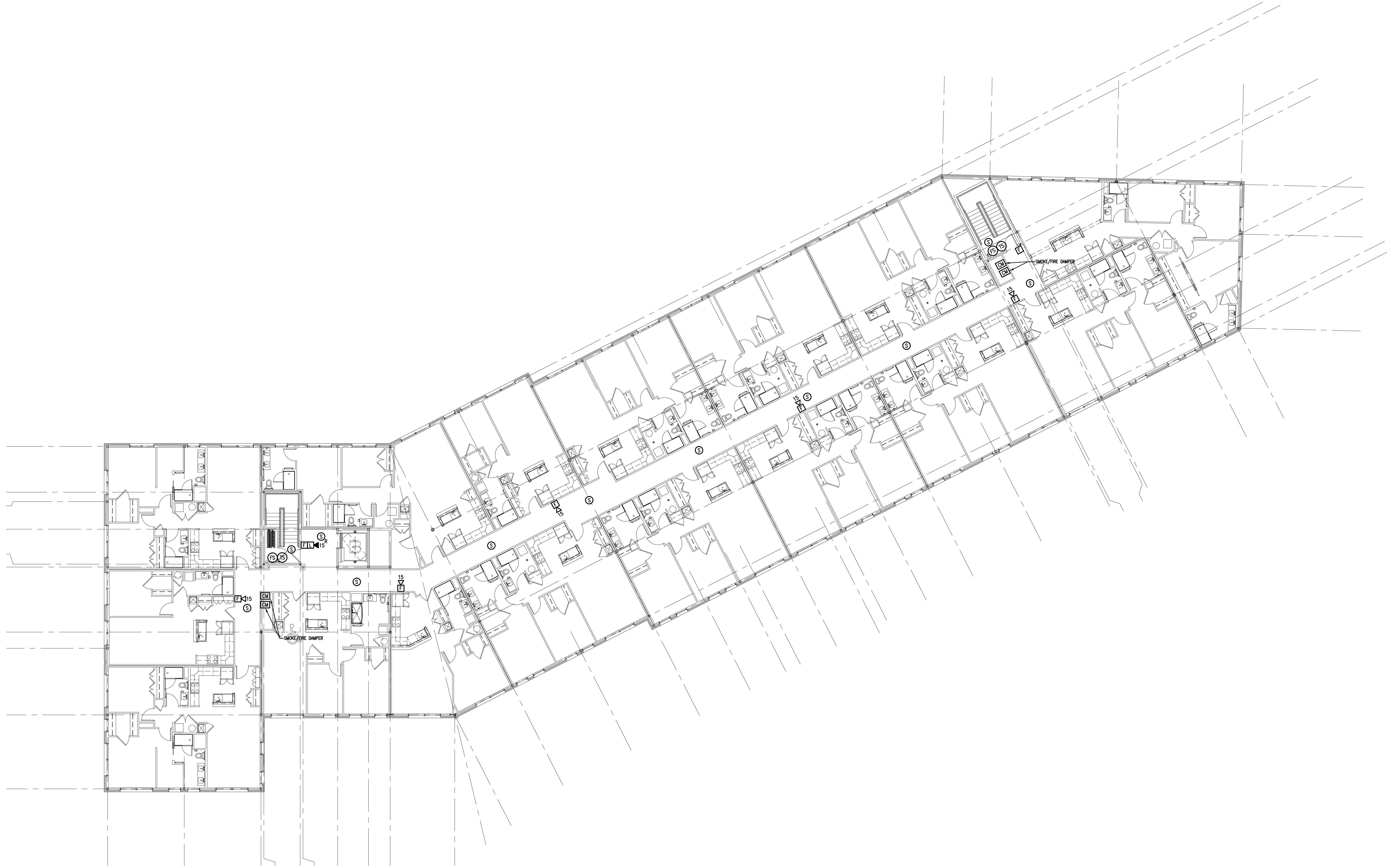
1 ELECTRICAL -Fifth Level Fire Alarm Plan SCALE: 3/32"= 1'-0"
