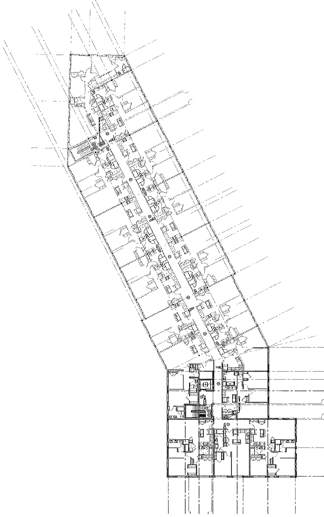
1 ELECTRICAL - 5th Level Fire Alarm Plan SCALE: 3/32" = 1'-0"
