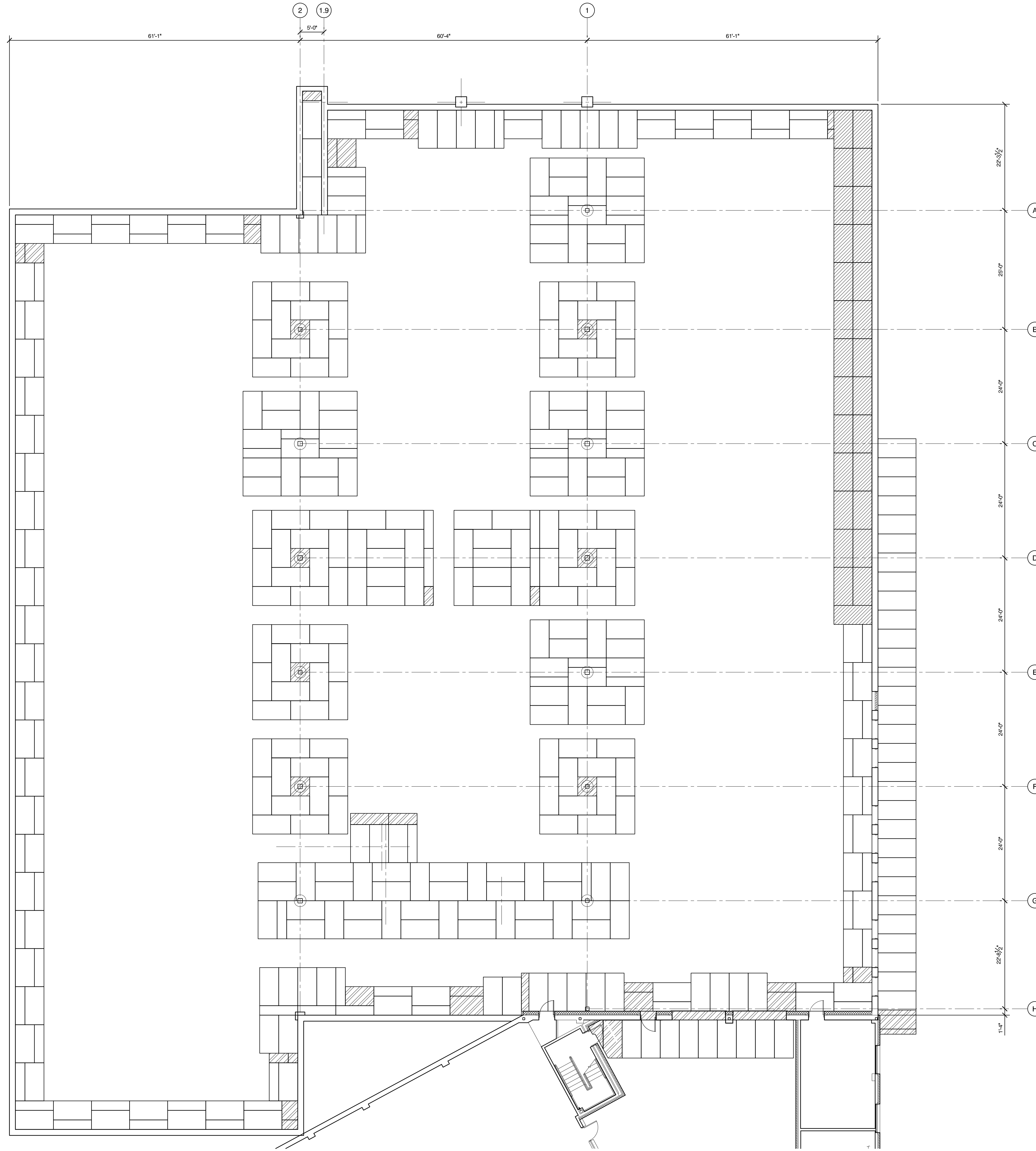
PLAN NORTH 1 PARKING GARAGE FOUNDATION INSULATION PLAN 3/32" = 1'-0"
