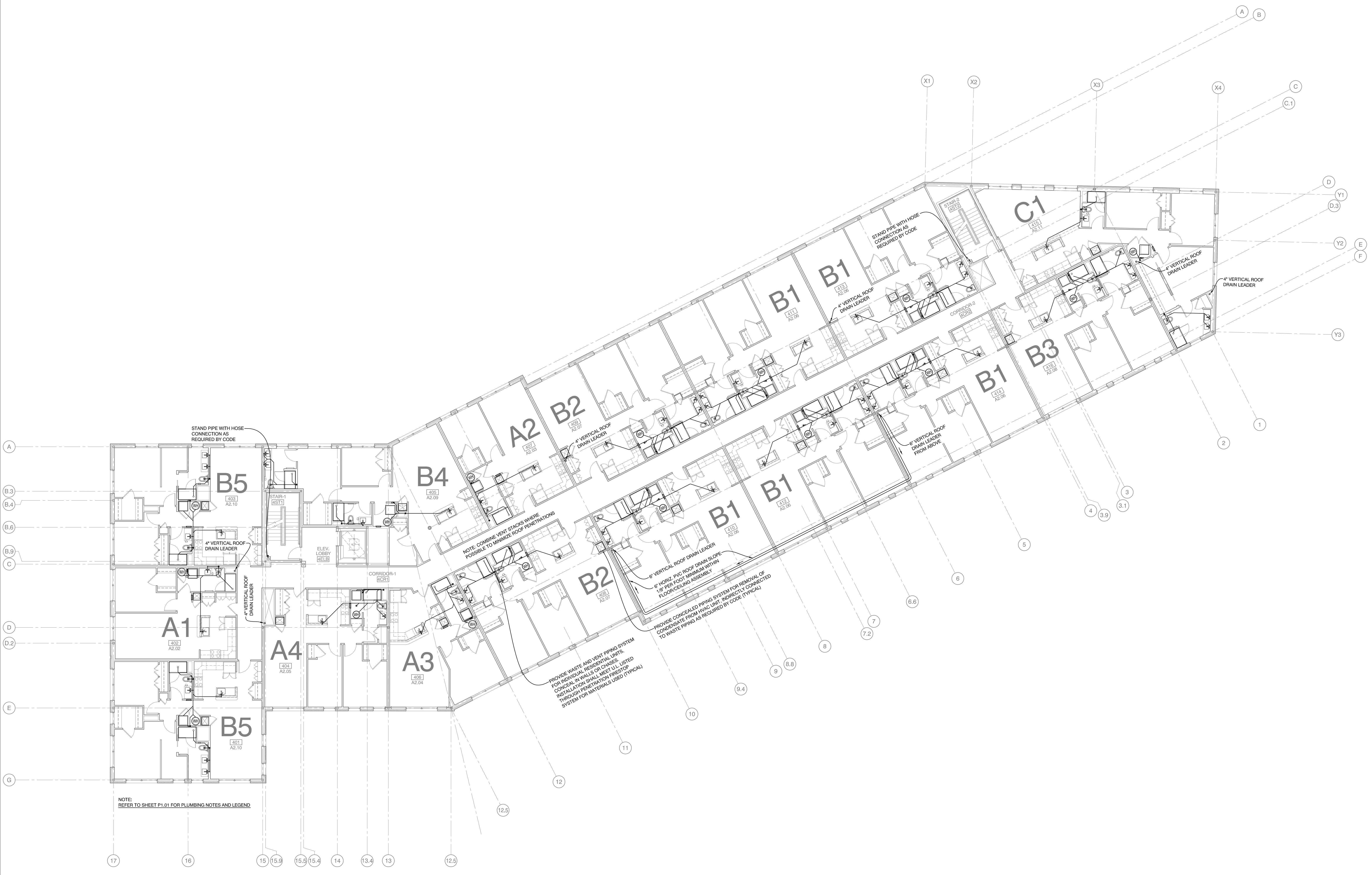
1 FOURTH LEVEL PLUMBING PLAN 3/32" = 1'-0"
