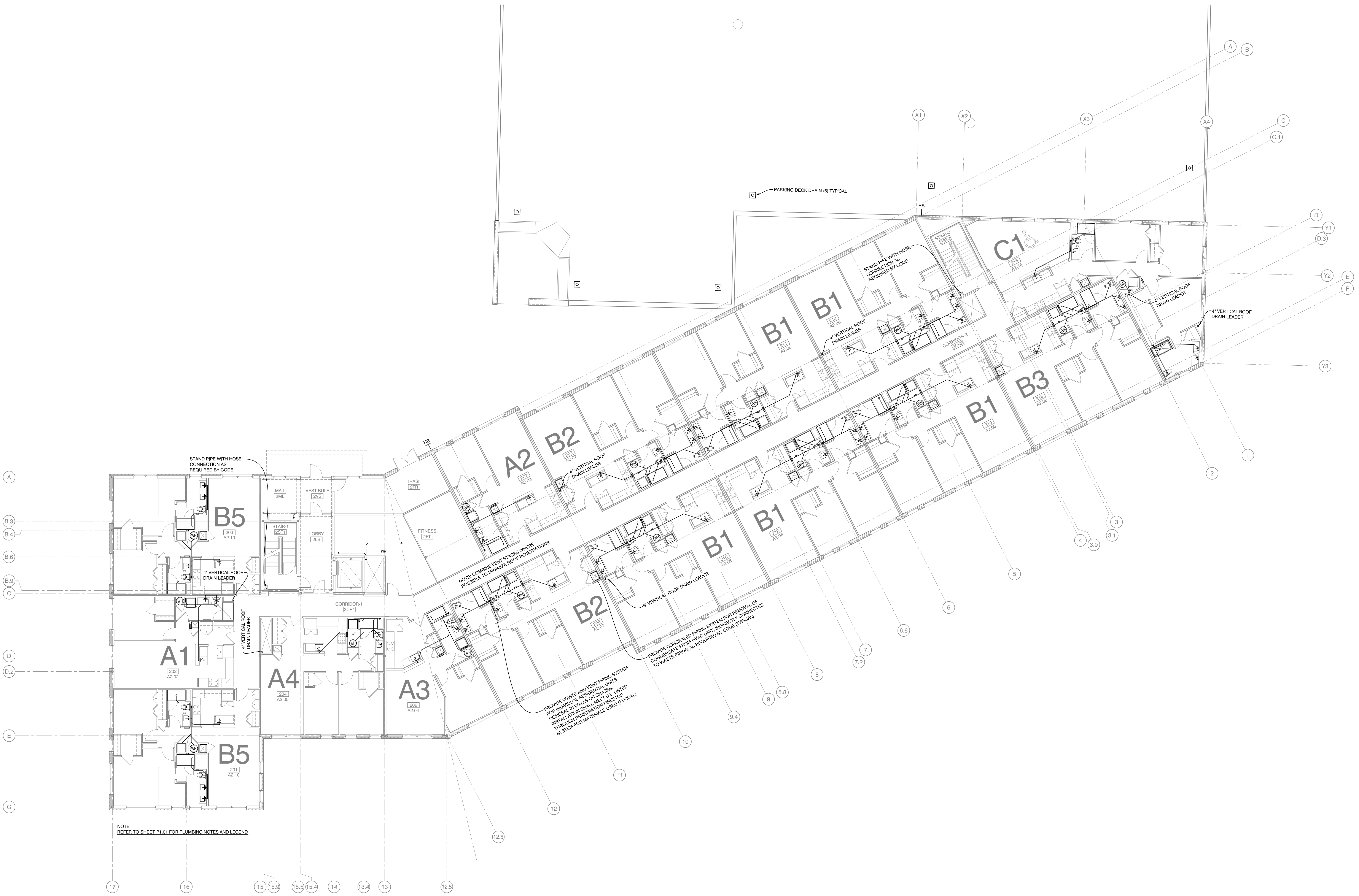
PLAN NORTH 1 SECOND LEVEL PLUMBING PLAN 3/32" = 1'-0"
