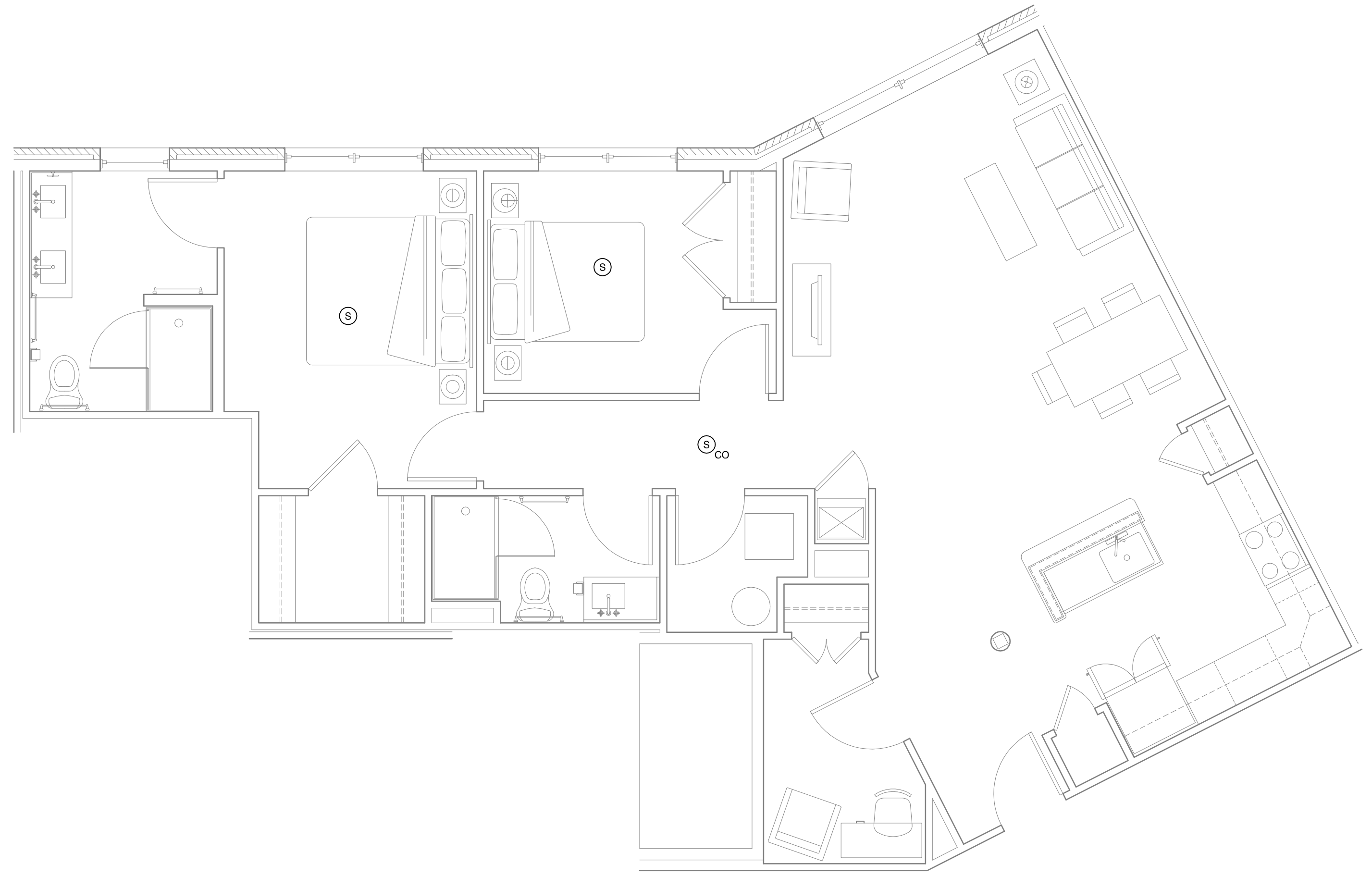
B4 2 BEDROOM UNIT FIRE ALARM PLAN 1/4" = 1'-0"; UNITS - 305, 405, & 505
