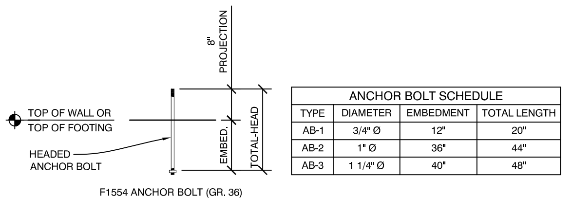
ANCHOR BOLTS 1/2" = 1'-0"
