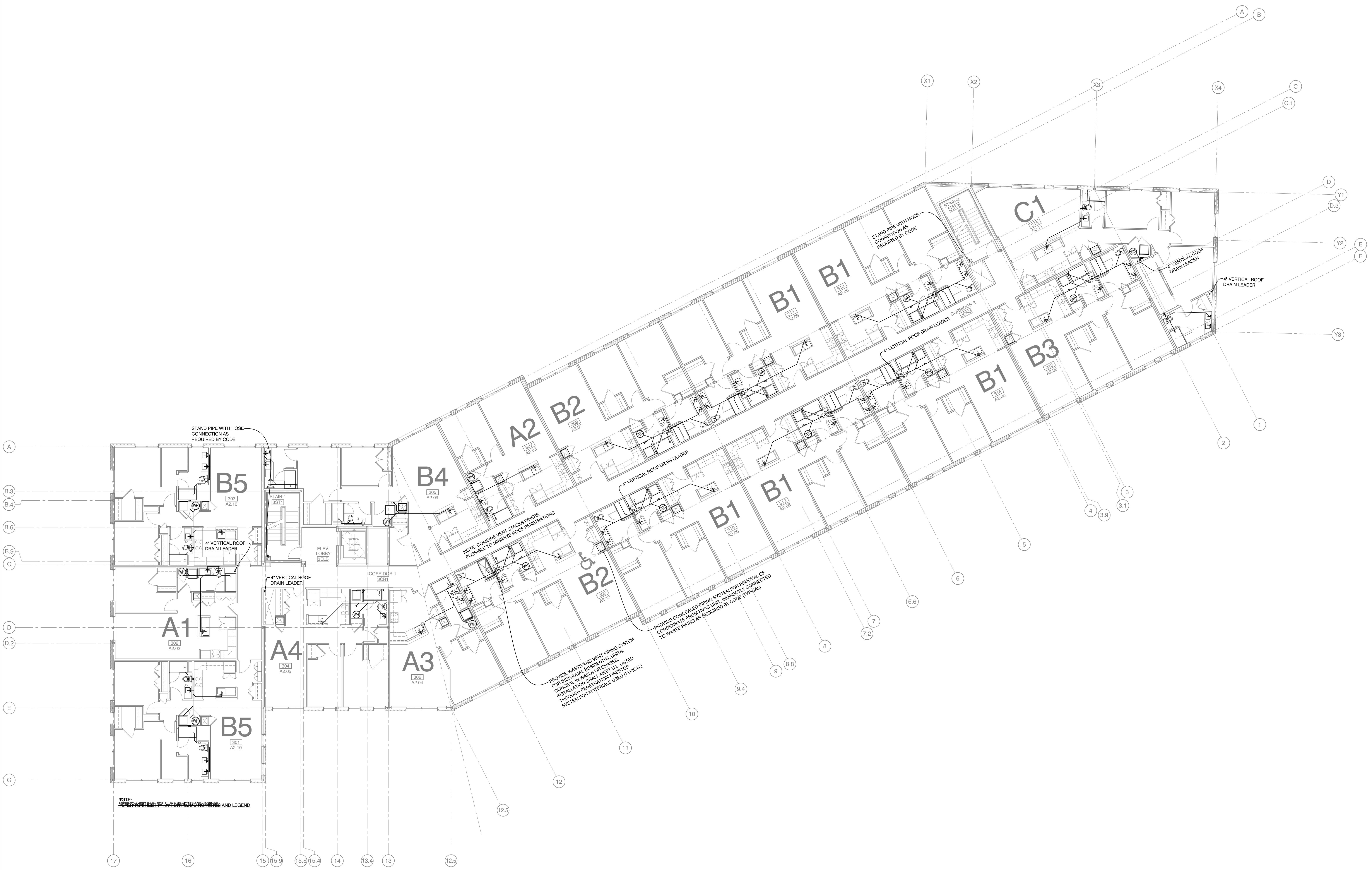
PLAN NORTH 1 THIRD LEVEL PLUMBING PLAN 3/32" = 1'-0"
