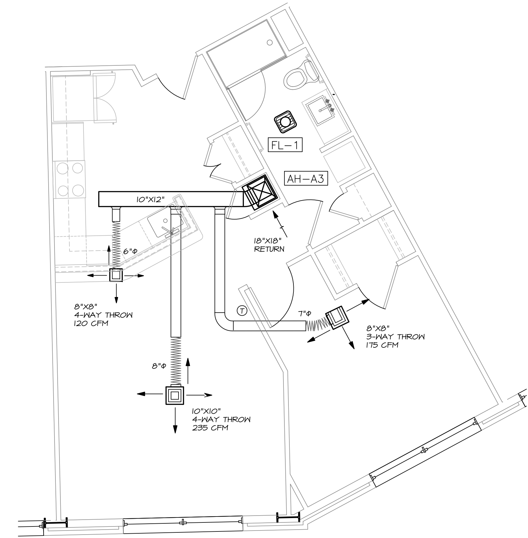
3 A3 UNIT DUCTWORK PLAN SCALE: 1/4" = 1'-0"
