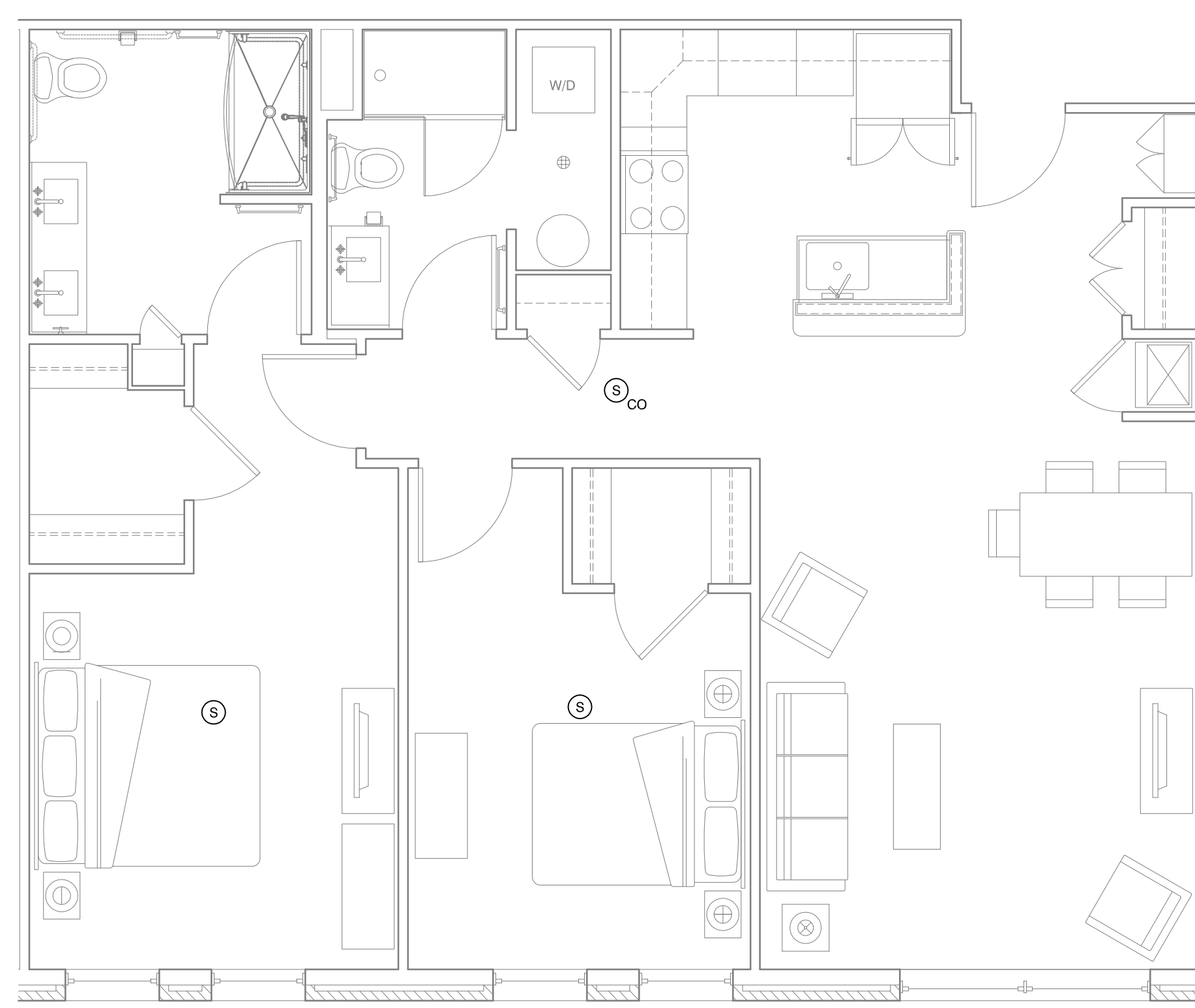
B2 2 BEDROOM ACCESSIBLE UNIT FIRE ALARM PLAN 1/4" = 1'-0"; UNIT 308
