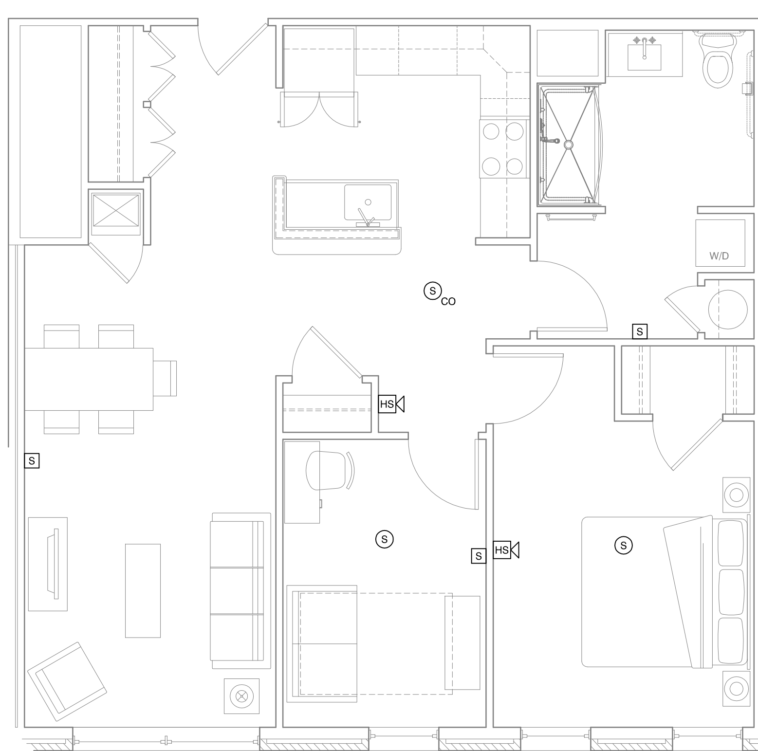
A4 1 BEDROOM ACCESSIBLE UNIT FIRE ALARM PLAN 1/4" = 1'-0"; UNIT 504
