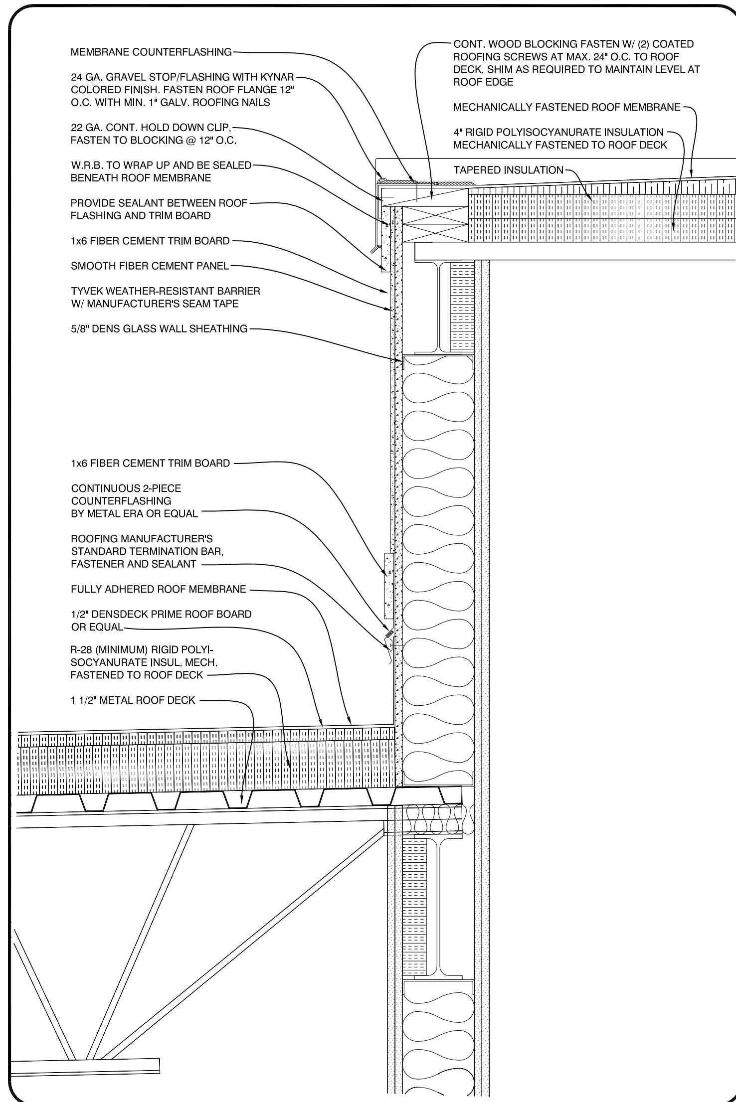
ROOF DETAIL SCALE: 1 1/2" = 1'-0"
