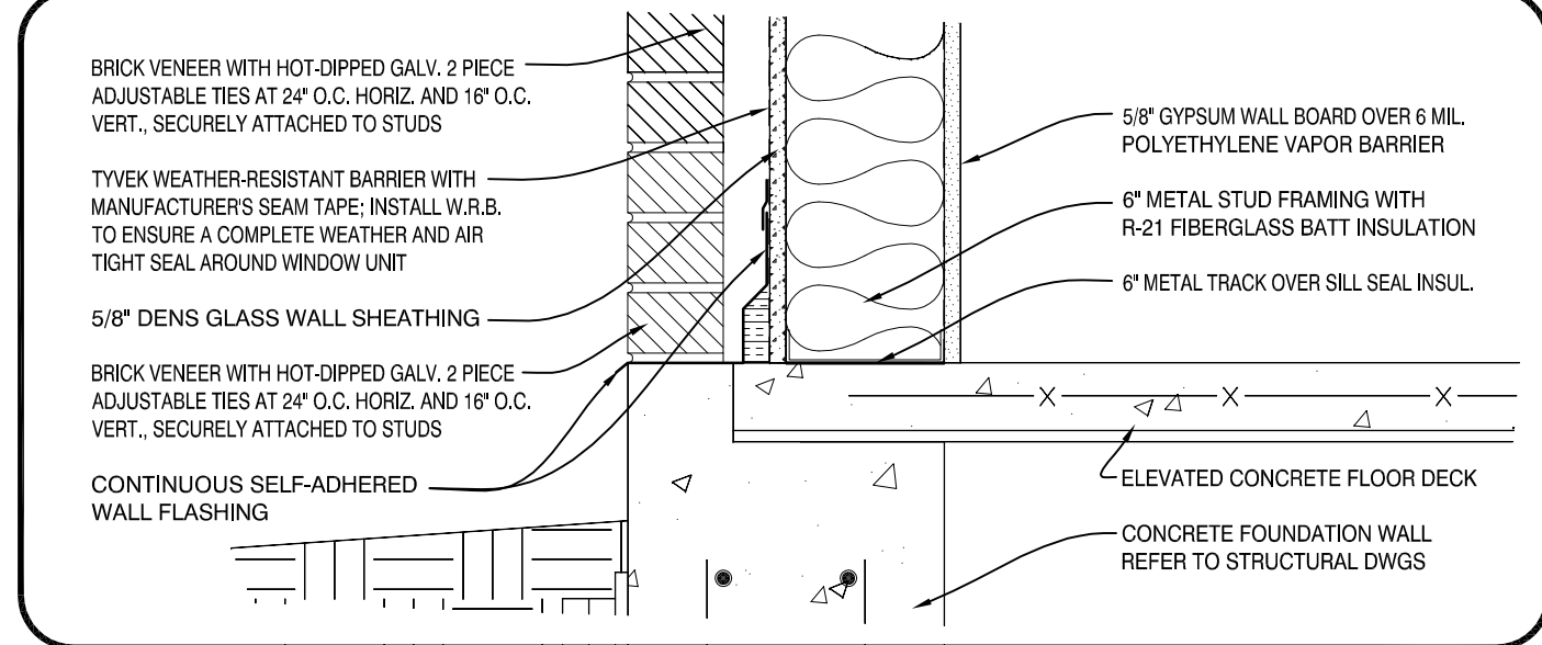
WALL BASE DETAIL SCALE: 1 1/2" = 1'-0"
