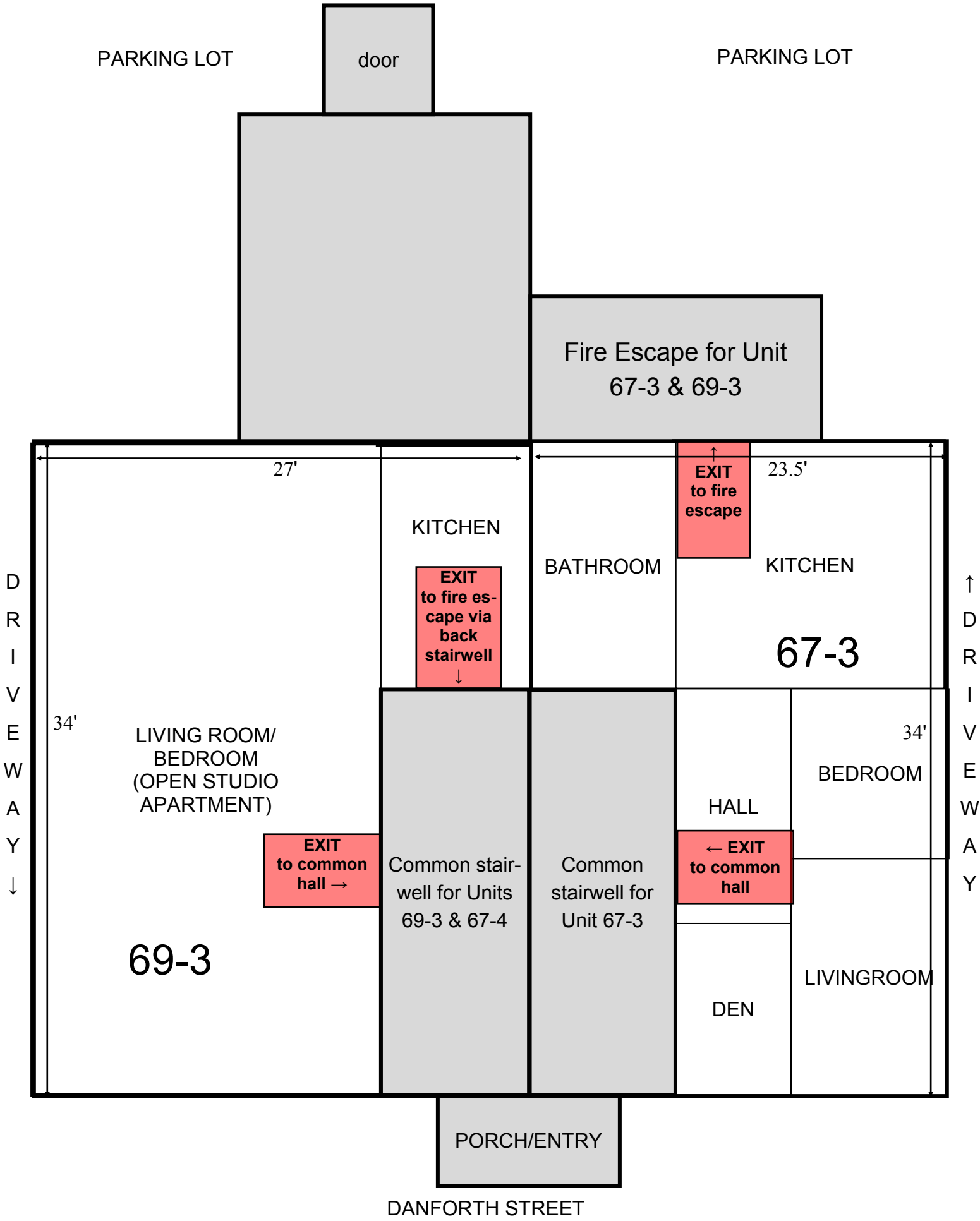
67/69 BIRD'S EYE VIEW: THIRD FLOOR
