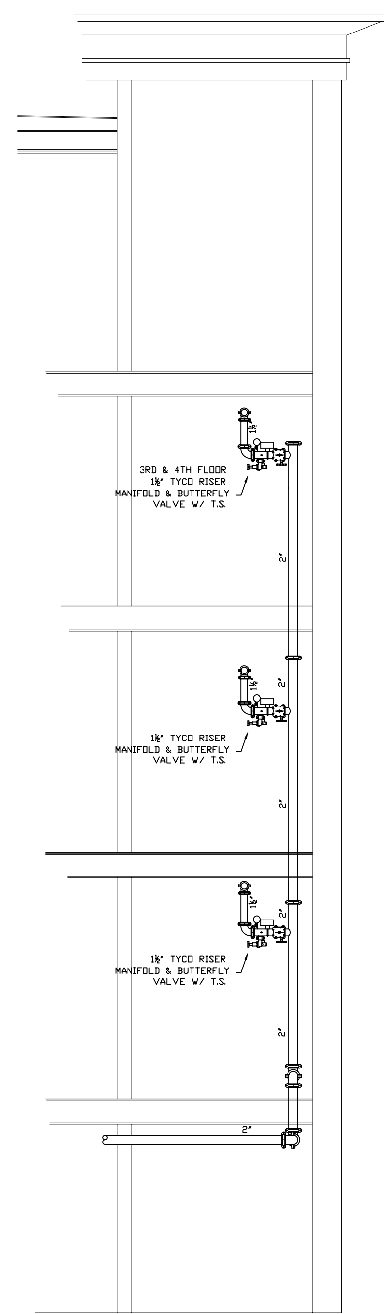
STAIR #1 WET RISER WITH FLOOR CONTROL VALVES SCALE: 1/4"=1'-0"
