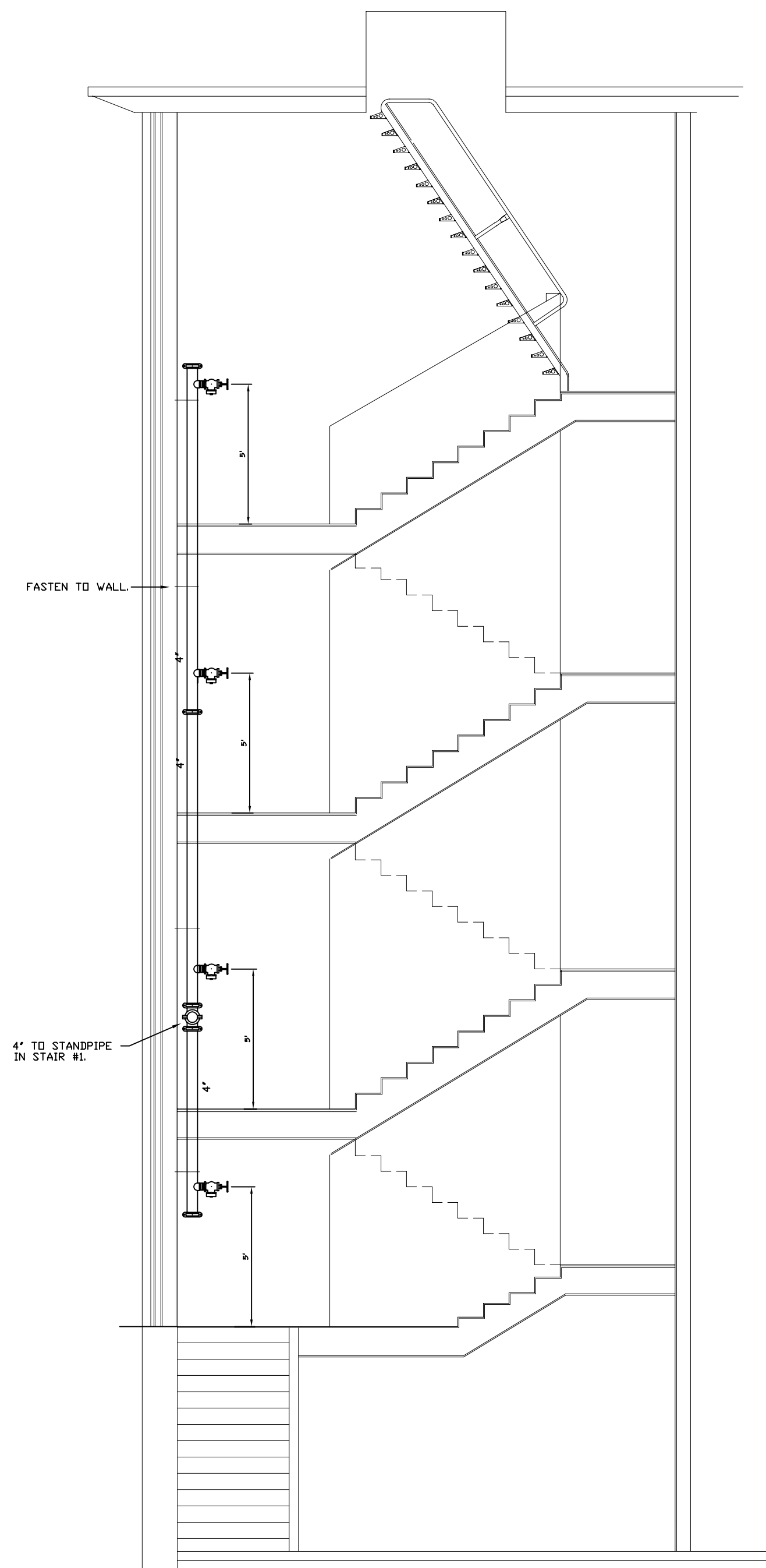
STAIR #1 MANUAL WET STAND PIPE WITH HOSE VALVES. SCALE: 1/4"=1'-0"
