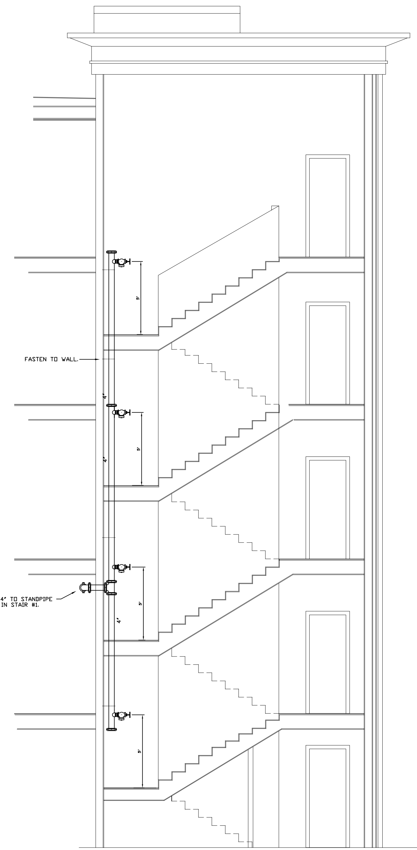
STAIR #2 MANUAL WET STAND PIPE WITH HOSE VALVES. SCALE: 1/4"=1'-0"
