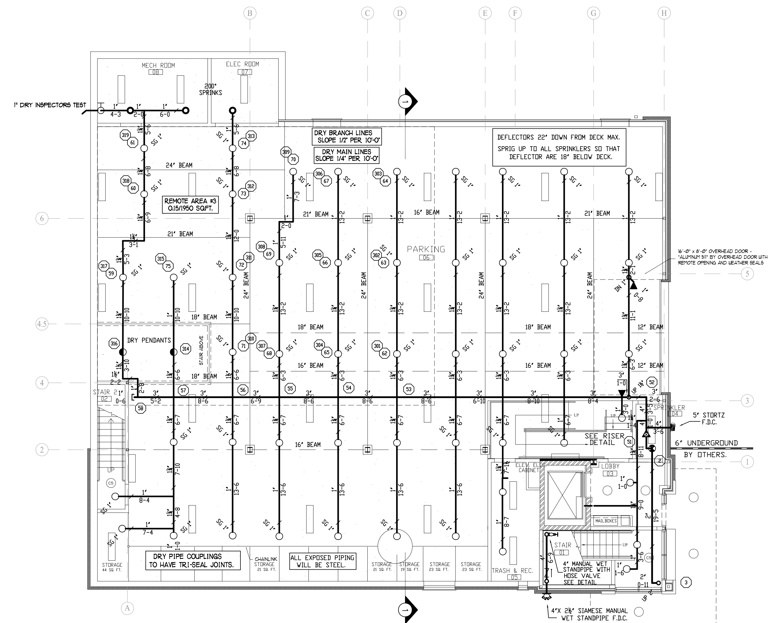
BASEMENT FIRE PROTECTION
