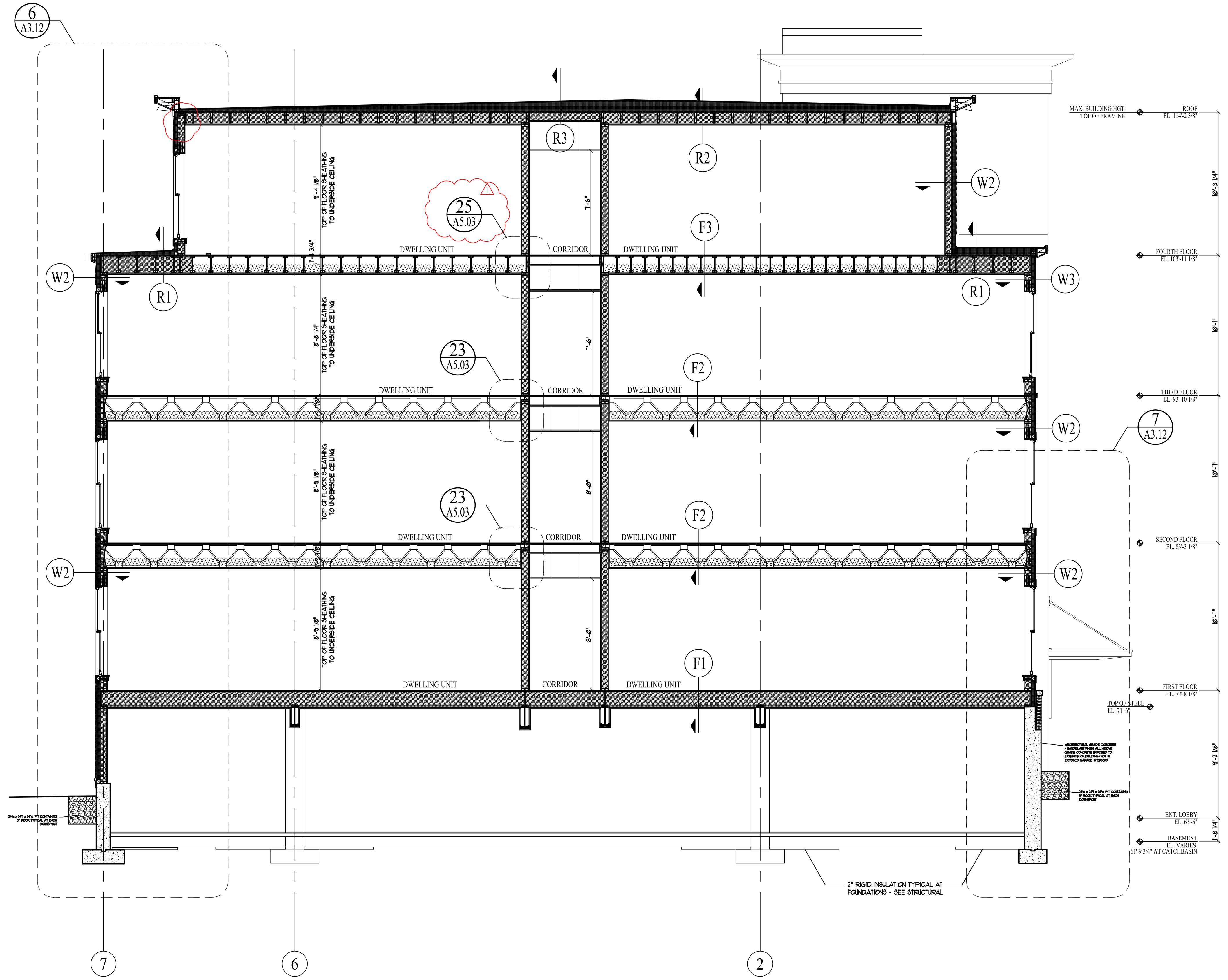
2 | BUILDING SECTION SCALE: 1/4"=1'-0"
