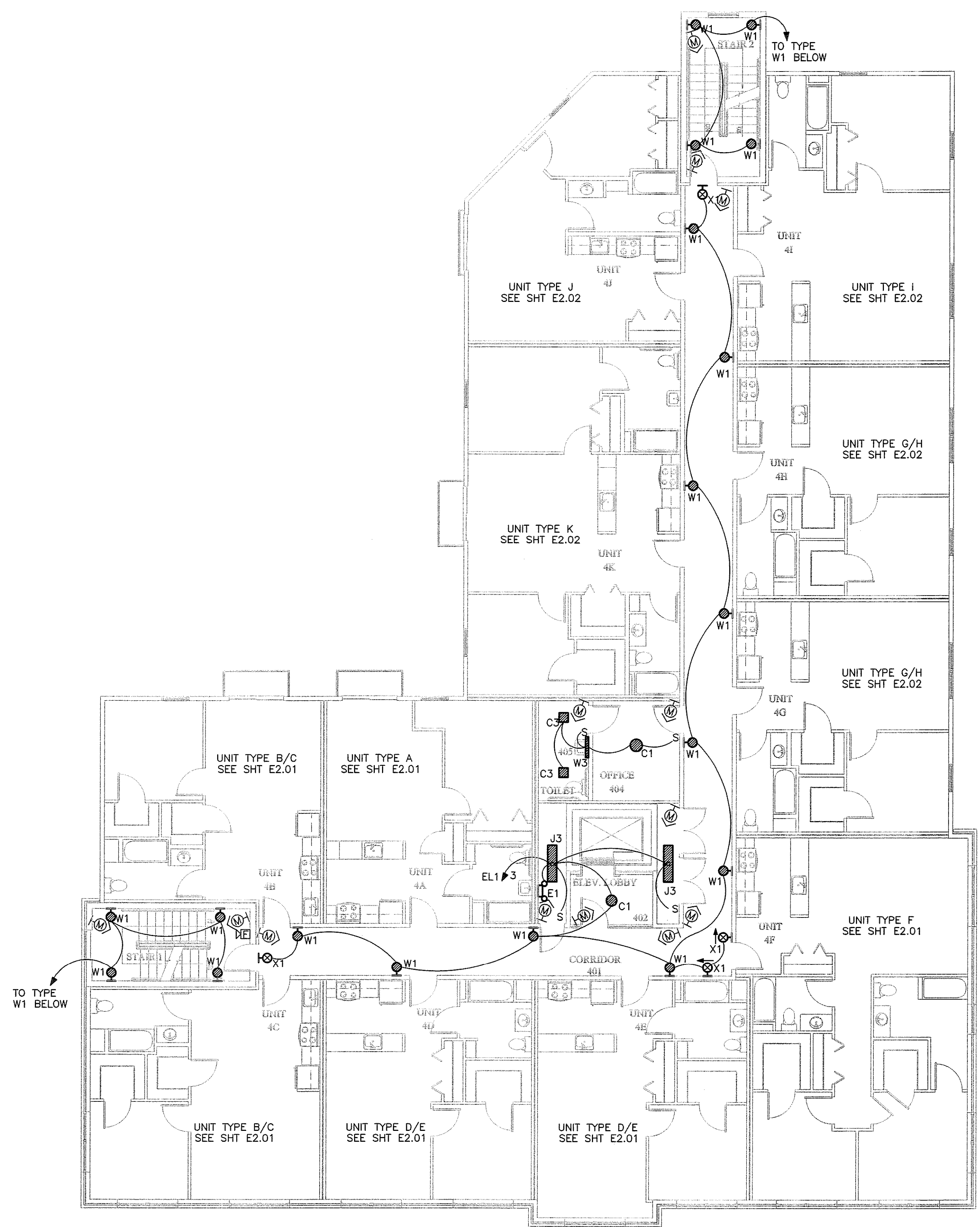
FOURTH FLOOR LIGHTING PLAN 1/8" = 1'-0"
