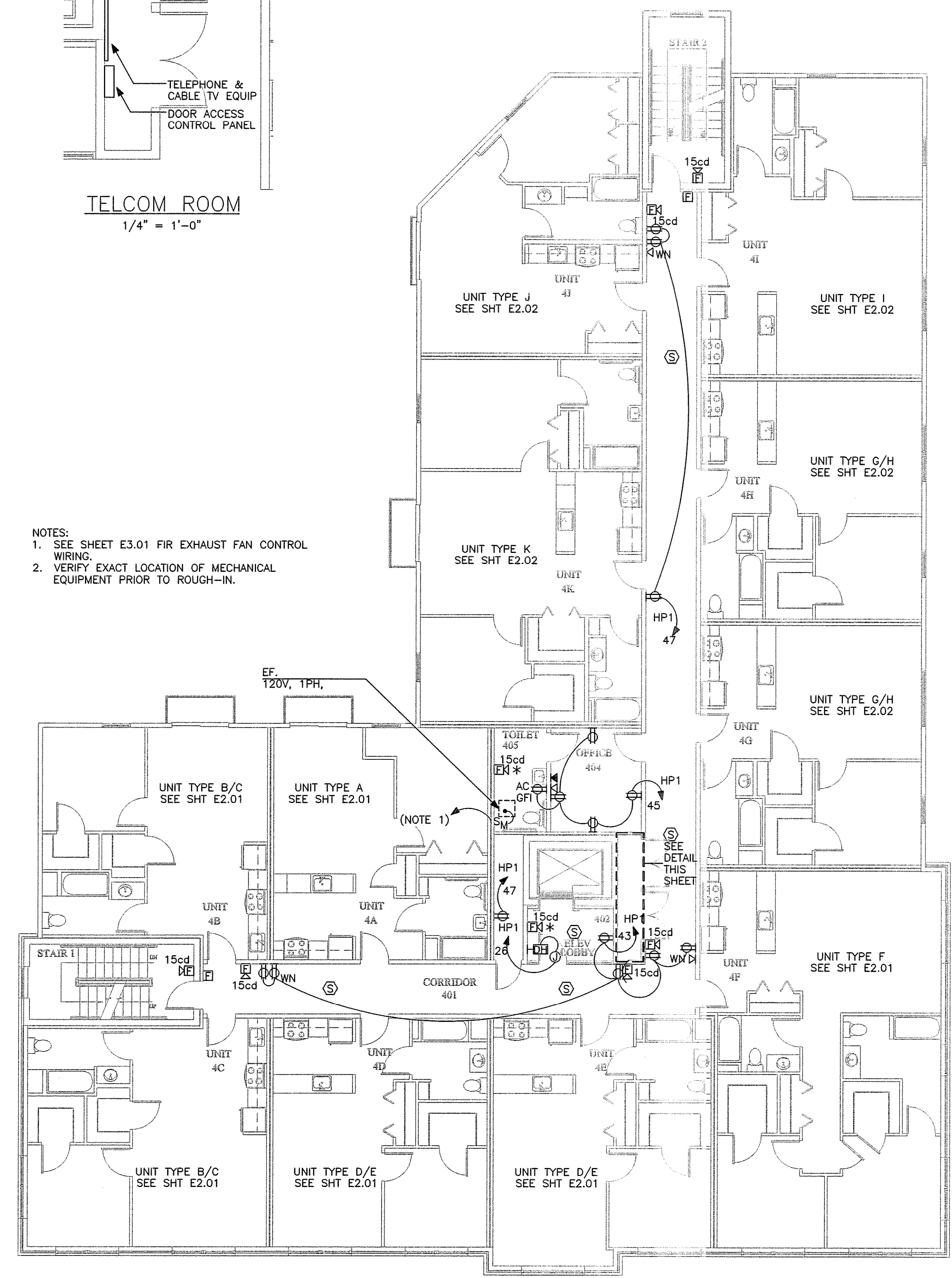
FOURTH FLOOR POWER PLAN 1/8" = 1'-0"
