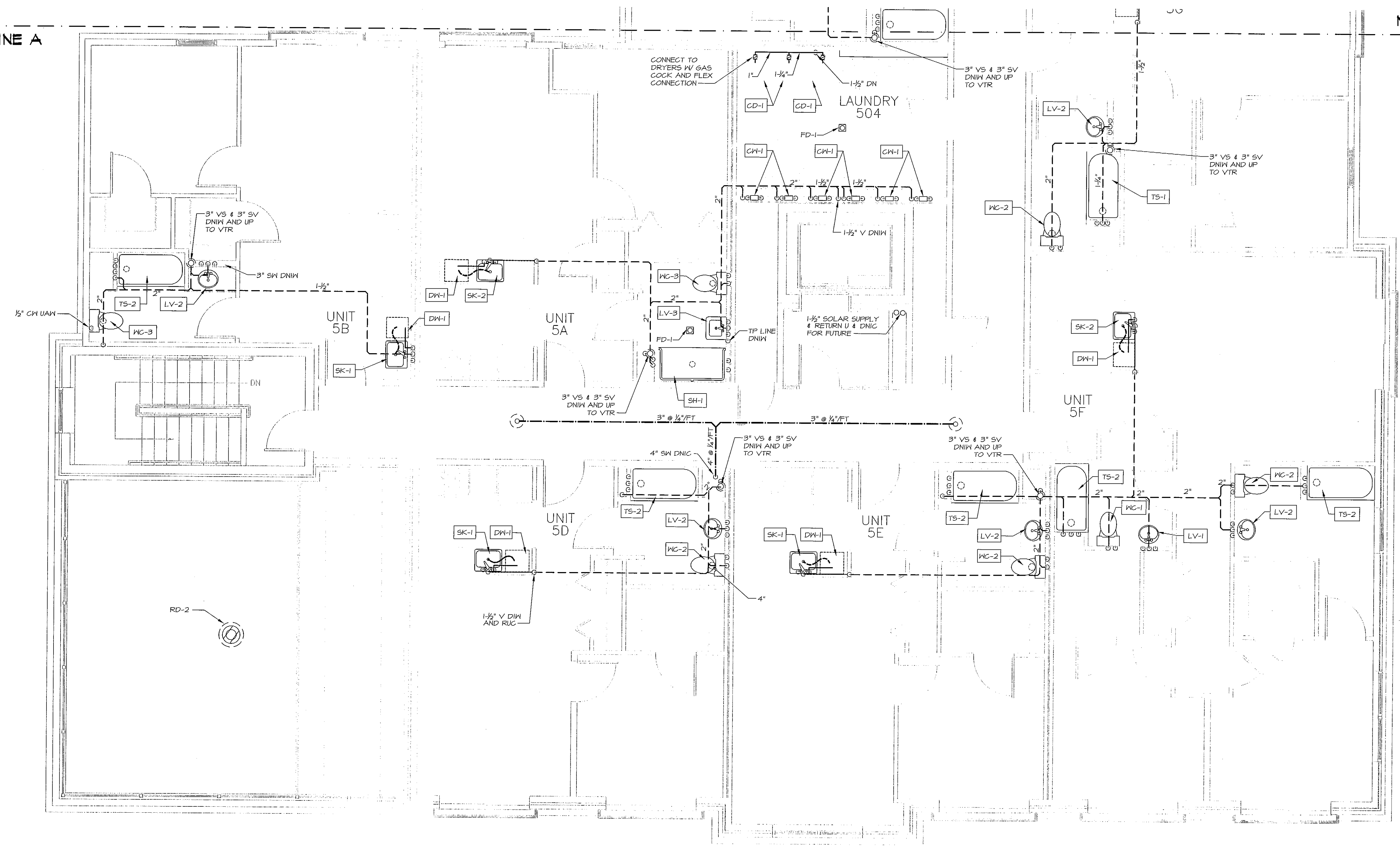
PLUMBING PLAN - FIFTH FLOOR SCALE: 1/4" = 1'-0"
