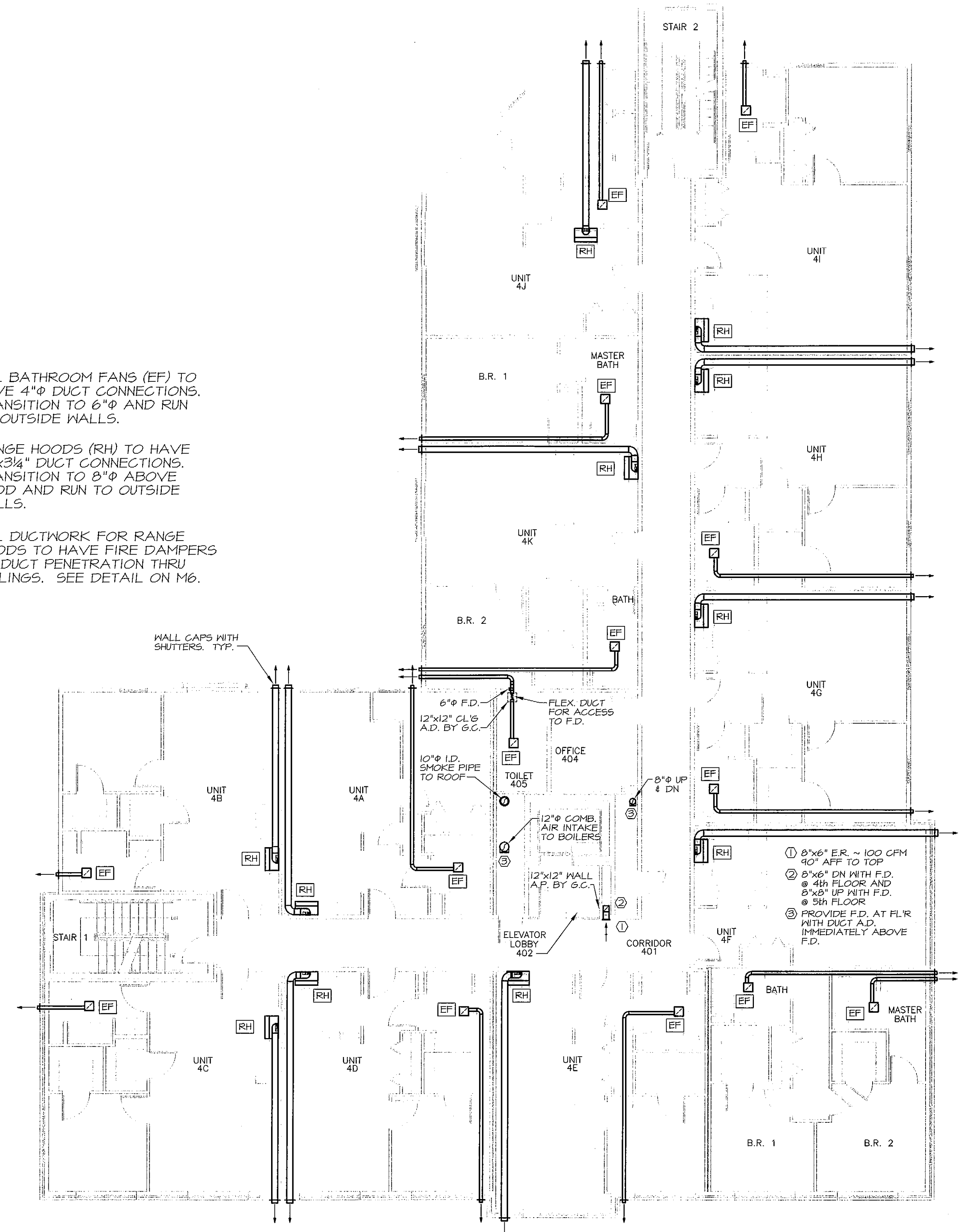
2 MECHANICAL FOURTH FLOOR PLAN SCALE: 1/8" = 1'-0"
