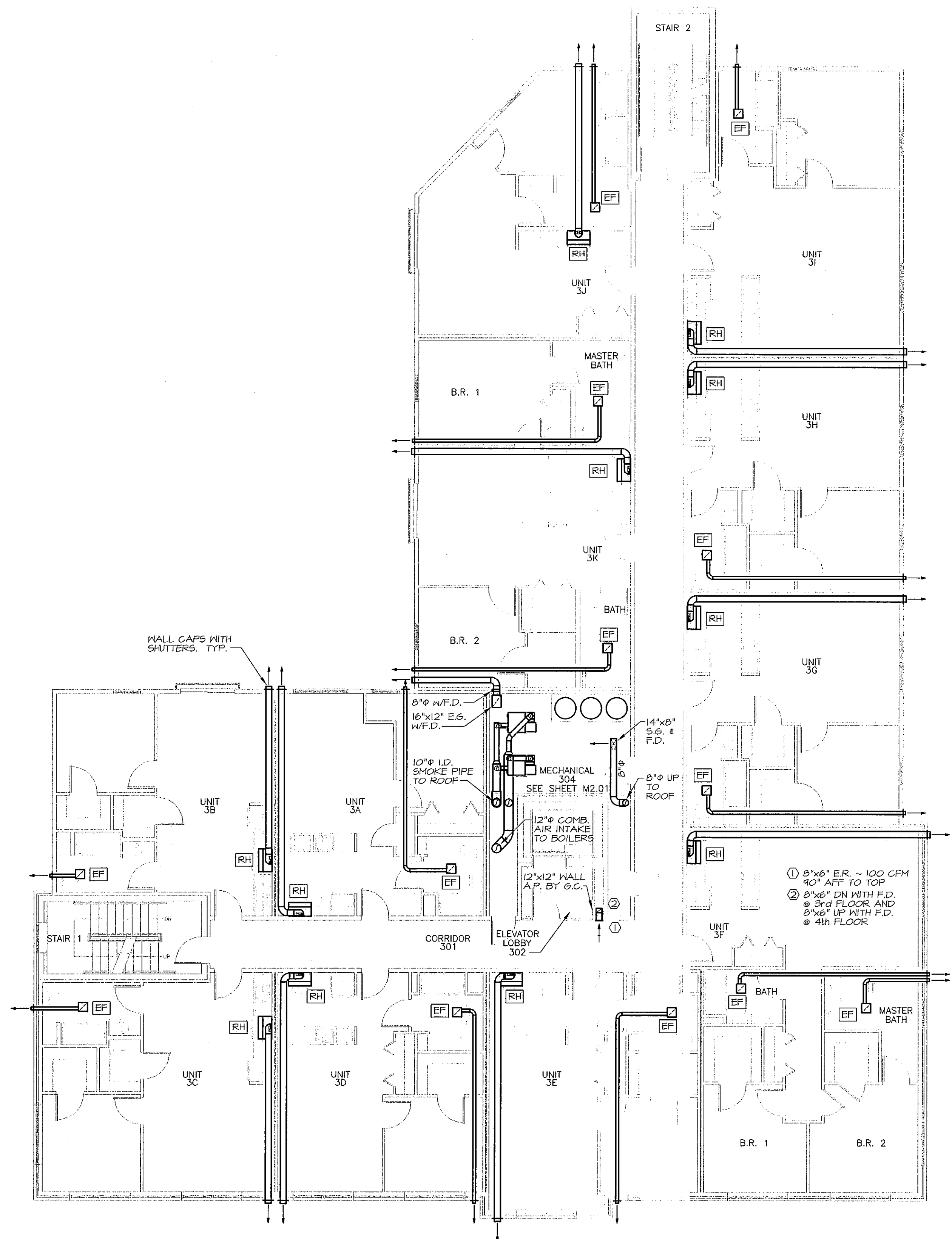
1 MECHANICAL THIRD FLOOR PLAN SCALE: 1/8" = 1'-0"
