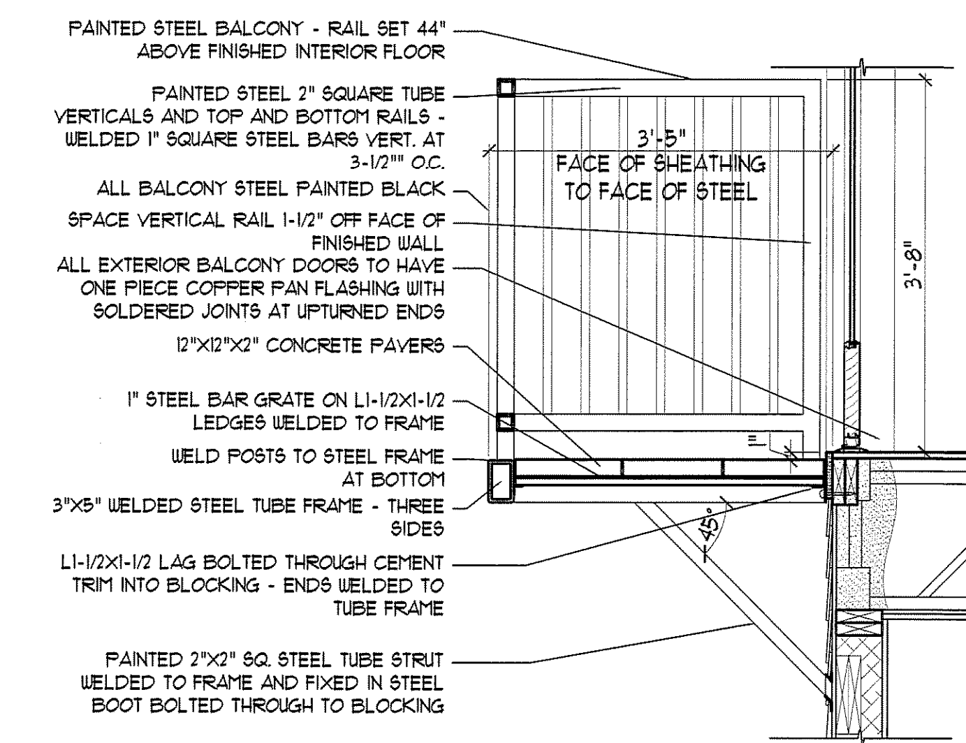
18 BALCONY DETAIL SCALE: 3/4"=1'-0"
