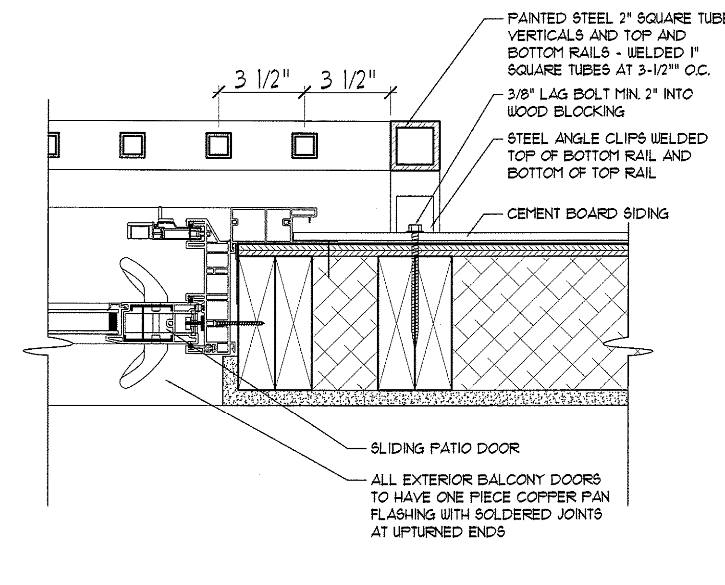
13 FRENCH BALCONY AT VINYL PATIO DOOR SCALE: 3/4"=1'-0"
