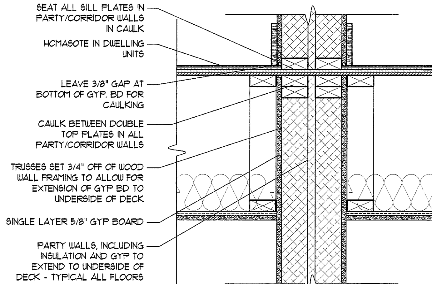
17 DETAIL AT TOP OF PARTY WALL SCALE: 1 1/2"=1'-0"
