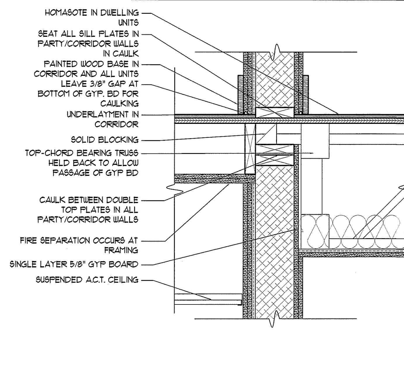
16 DETAIL AT CORRIDOR WALL/FLOOR INTERSECTION SCALE: 1 1/2"=1'-0"
