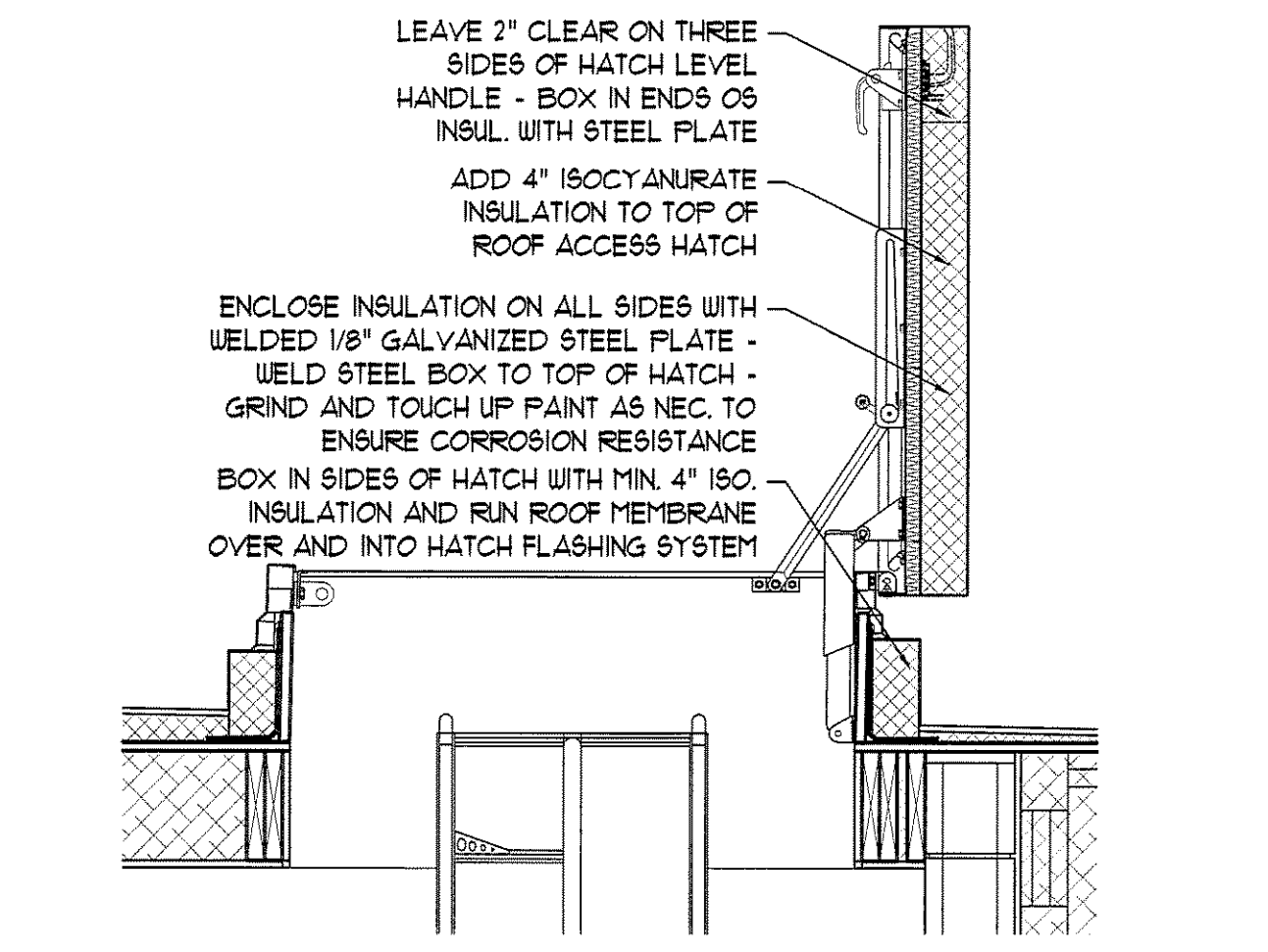
21 ROOF ACCESS HATCH DETAIL SCALE: 3/4"=1'-0"
