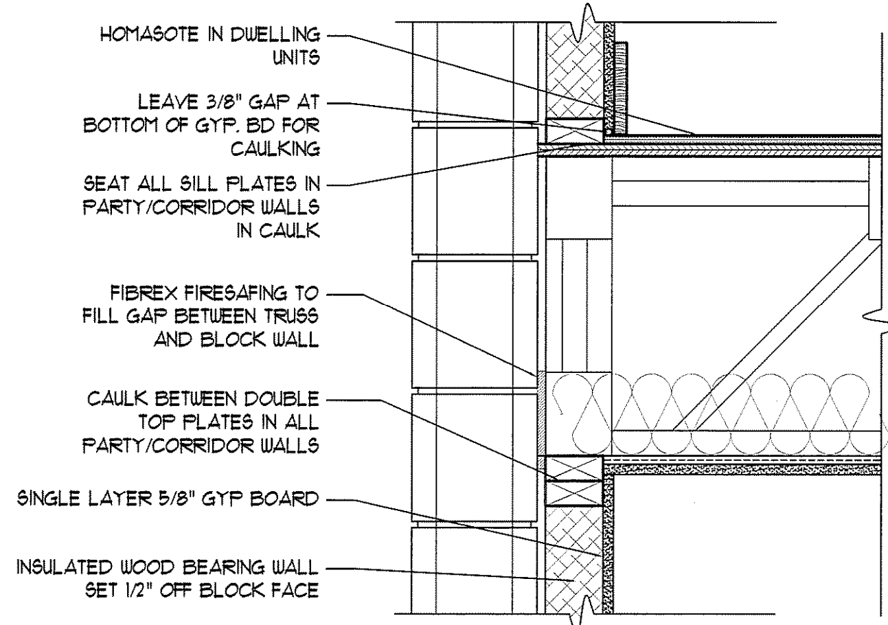
20 WOOD FRAMING FIRESTOPPING DETAIL SCALE: 1 1/2"=1'-0"
