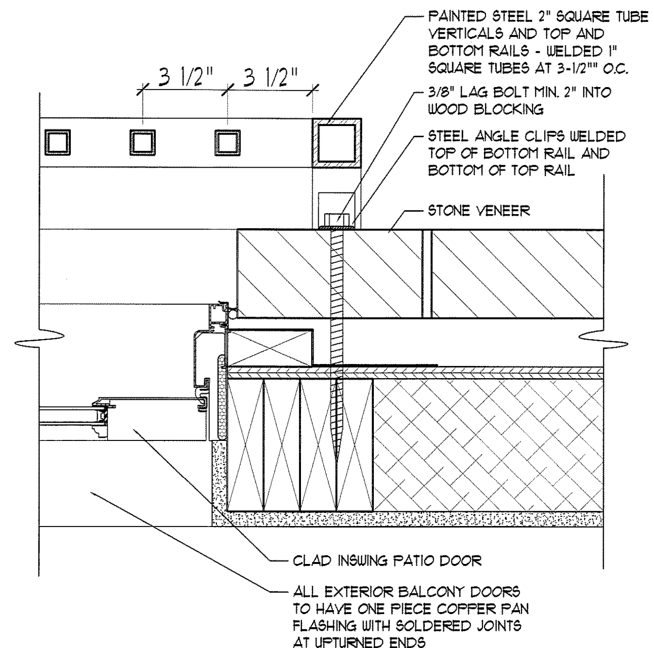
19 FRENCH BALCONY AT STONE VENEER SCALE: 3/4"=1'-0"
