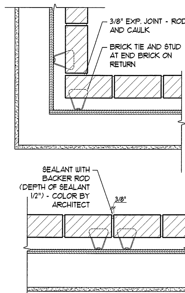
14 BRICK EXPANSION JOINT DETAILS SCALE: 1 1/2"=1'-0"
