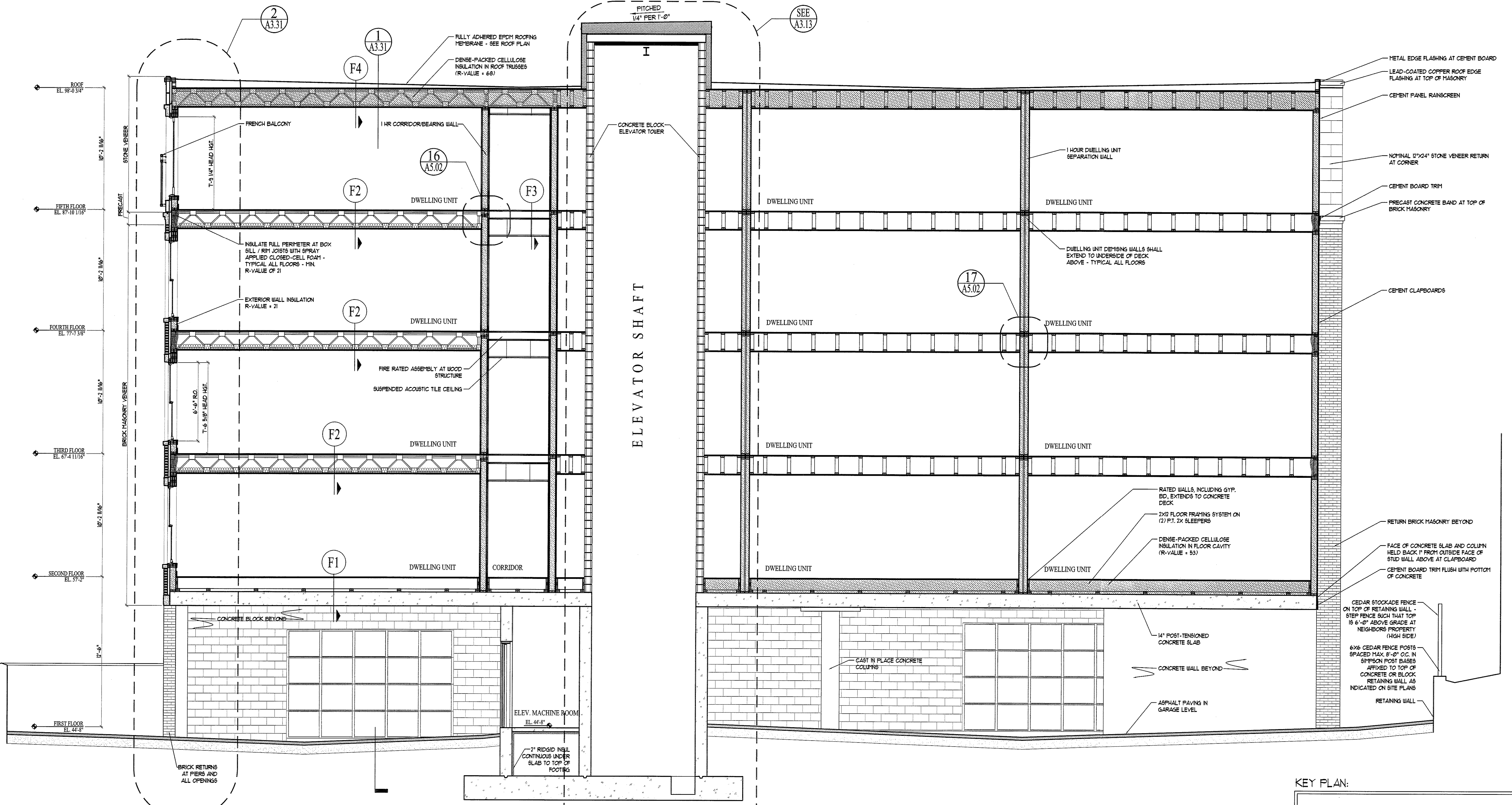
B BUILDING SECTION SCALE: 1/4" = 1'-0"
