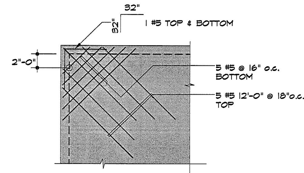
TRIM BARS AT SUPPORTED SLAB EDGES
