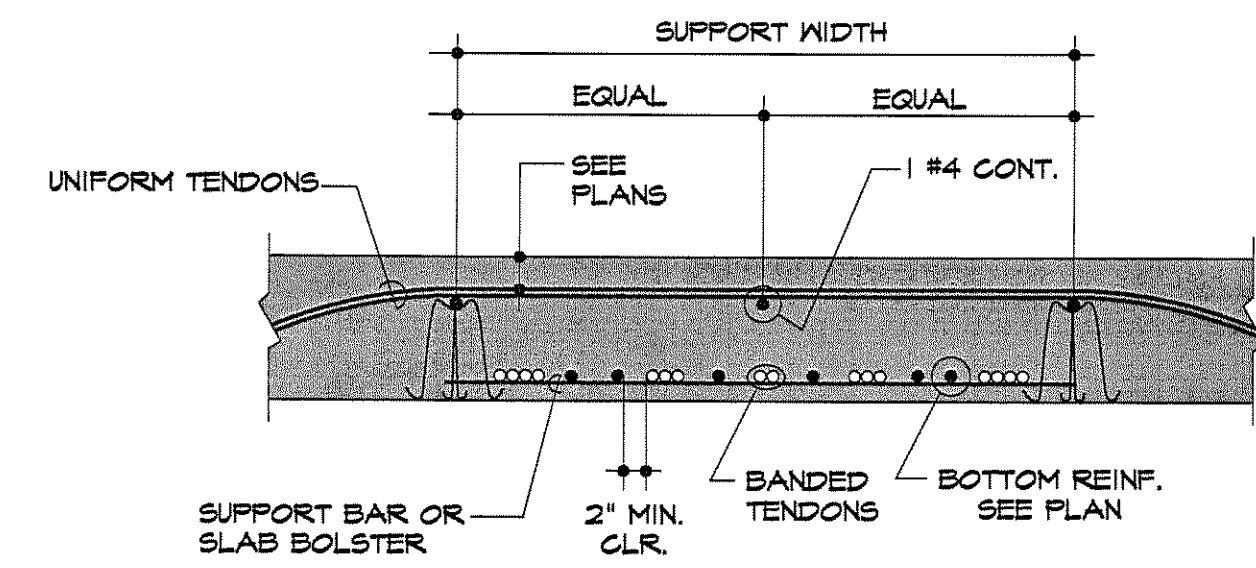
SECTION - BANDED TENDONS AT MID-SPAN
