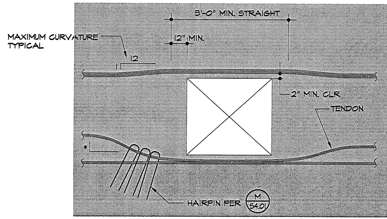
TENDON PLACEMENT AT OPENING 24" OR LARGER
