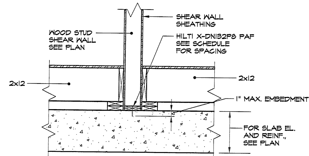
TYPICAL DETAIL OF STUD WALL HOLD-DOWN AT PT SLAB TYPE "A"
