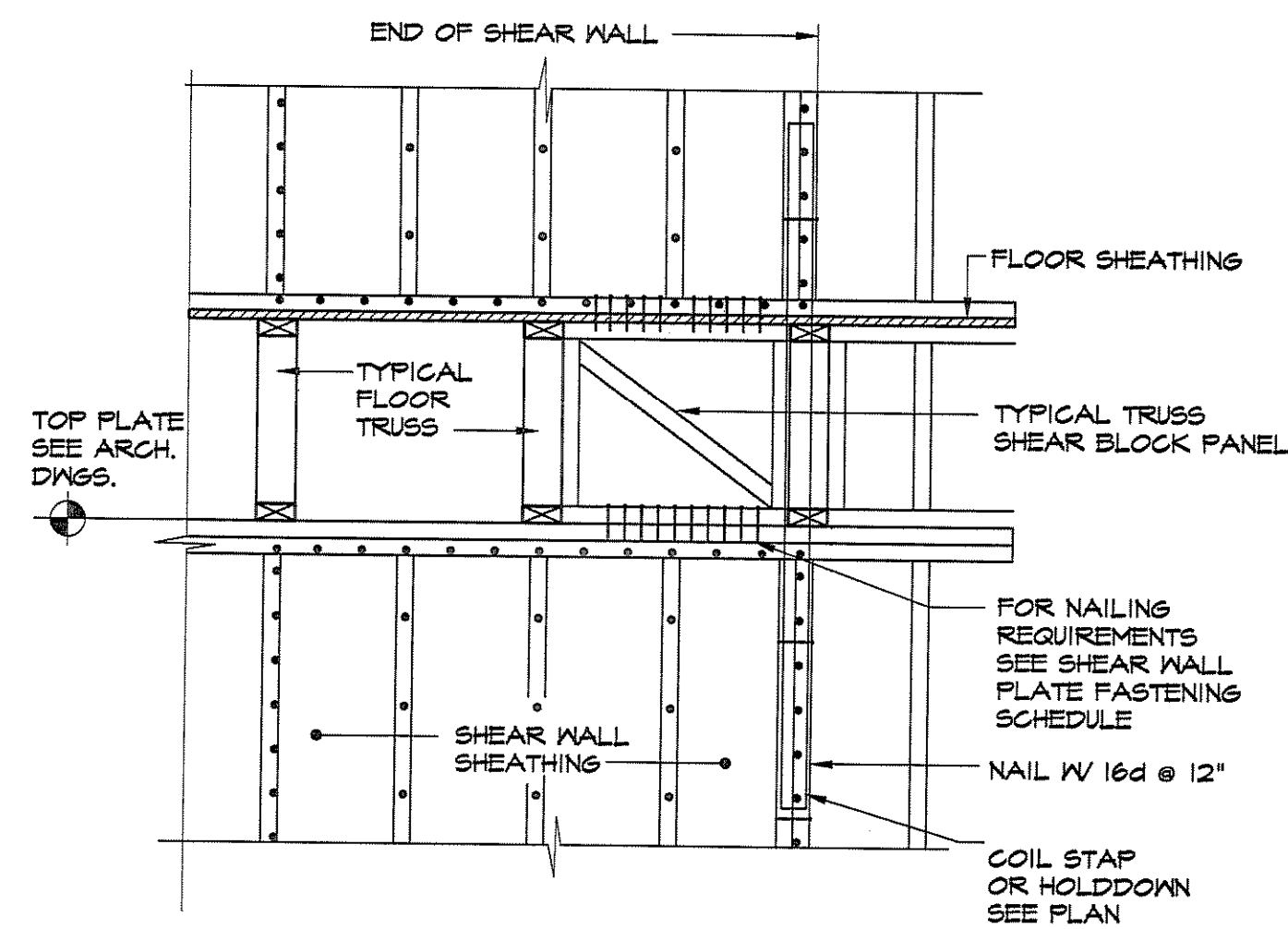
TYPICAL SHEAR WALL DETAIL AT TRUSS SHEAR BLOCK PANEL
