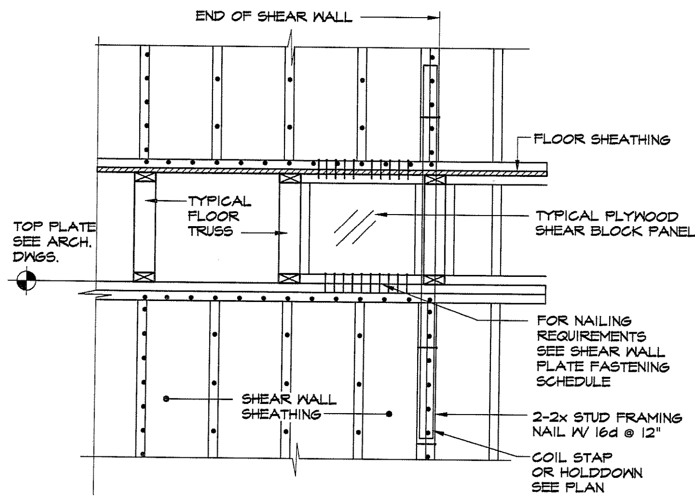
TYPICAL SHEAR WALL DETAIL AT PLYWOOD SHEAR BLOCK PANEL
