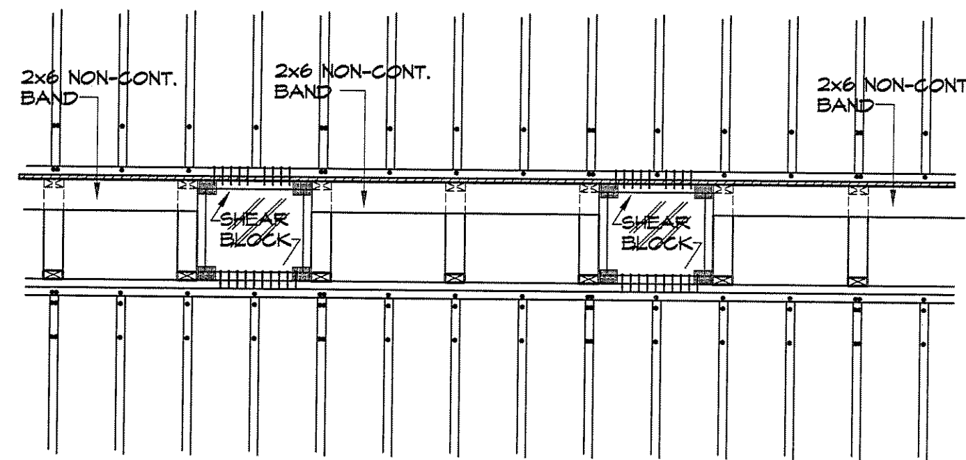
TYPICAL TRUSS END AT SHEAR PLATE
