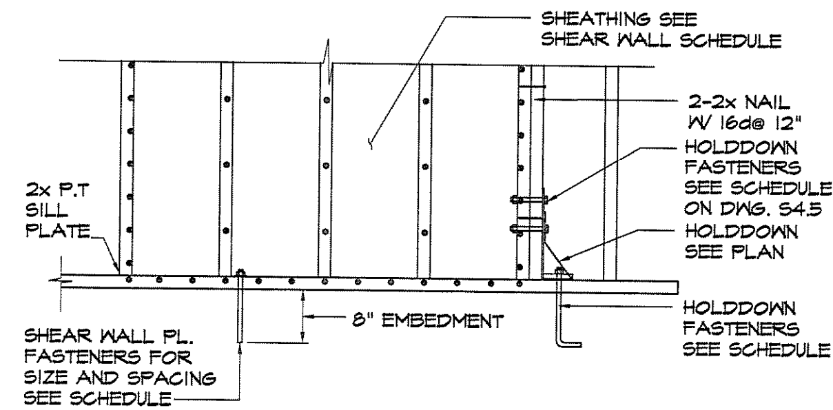
TYPICAL SHEAR WALL DETAIL AT ANCHORAGE
