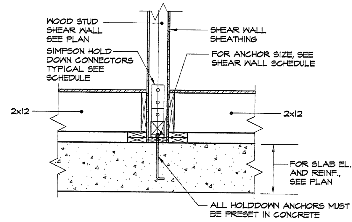
TYPICAL DETAIL OF STUD WALL HOLD-DOWN AT PT SLAB TYPE "A"
