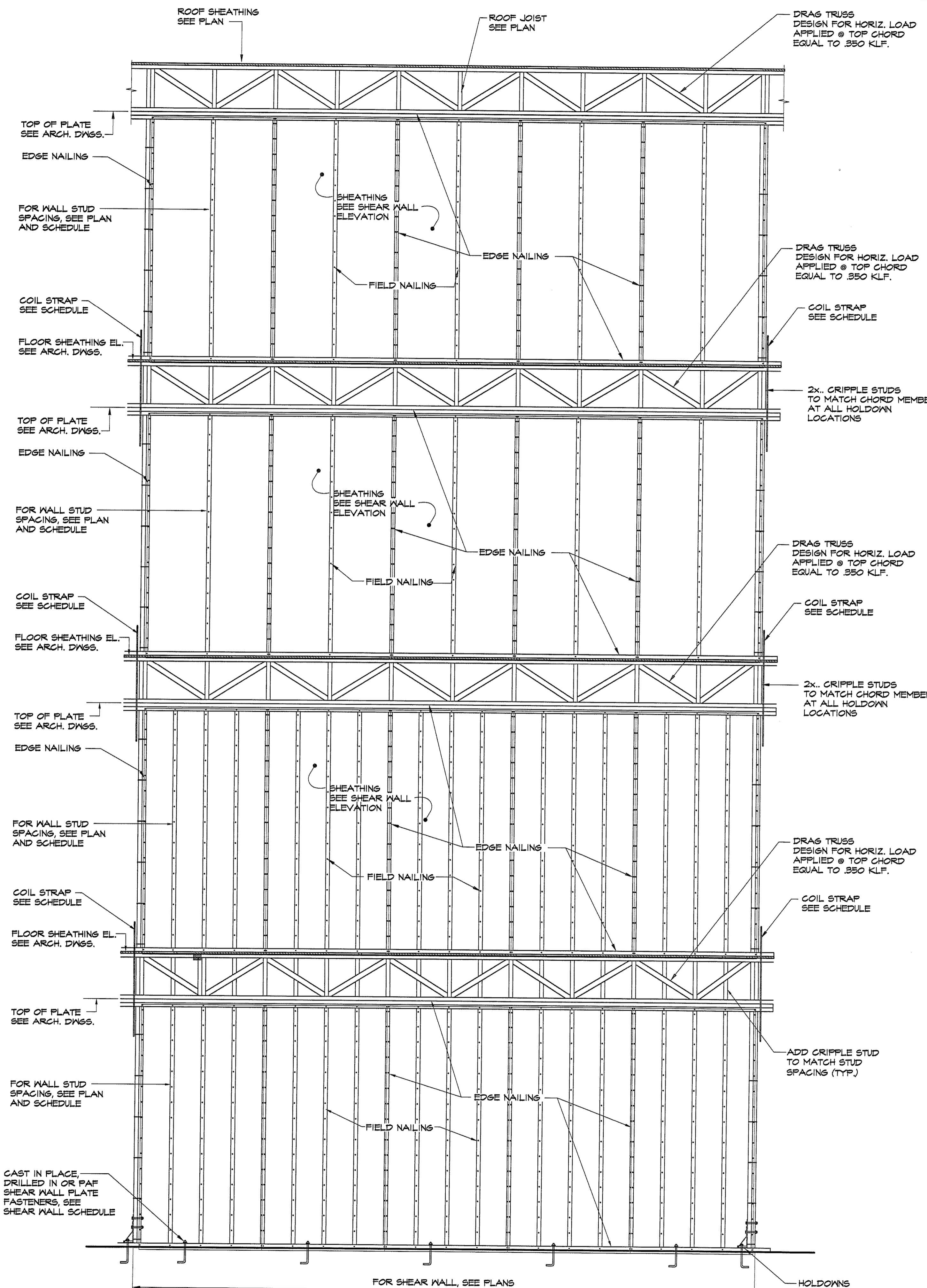
TYPICAL SHEAR WALL ELEVATION PARALLEL TO TRUSSES
