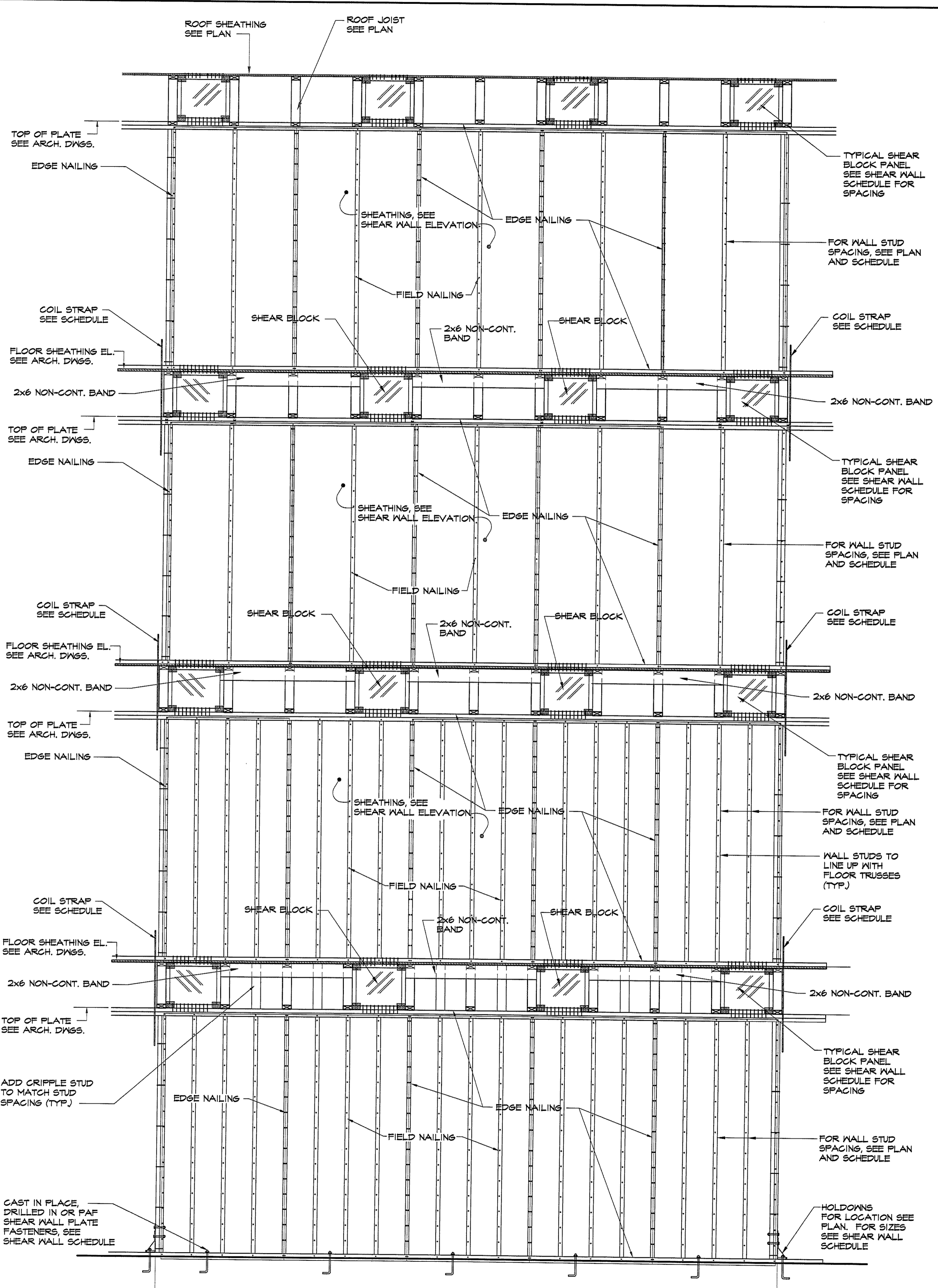
TYPICAL SHEAR WALL ELEVATION PERPENDICULAR TO TRUSSES
