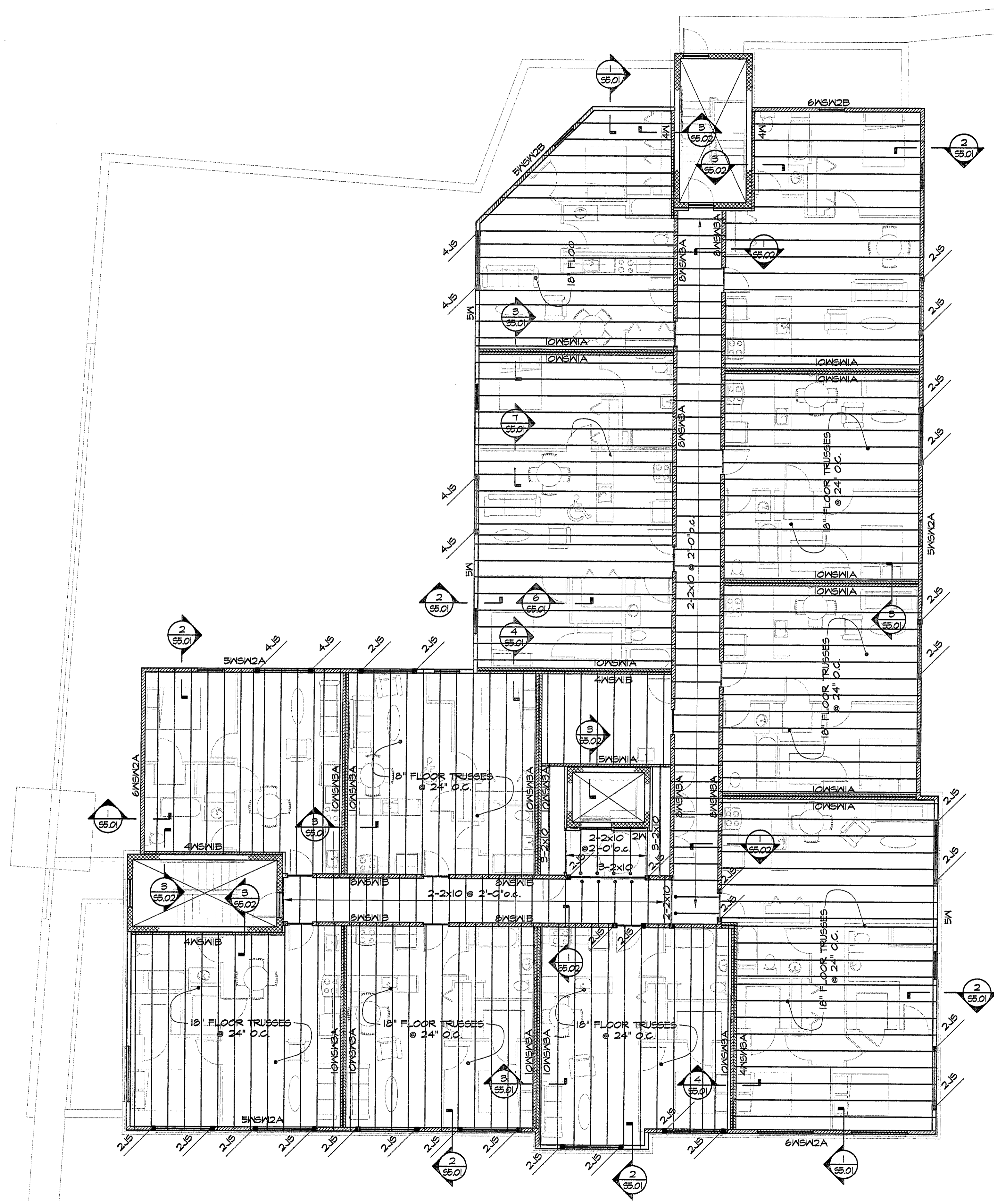
THIRD FLOOR FRAMING PLAN 1/8"=1'-0"
