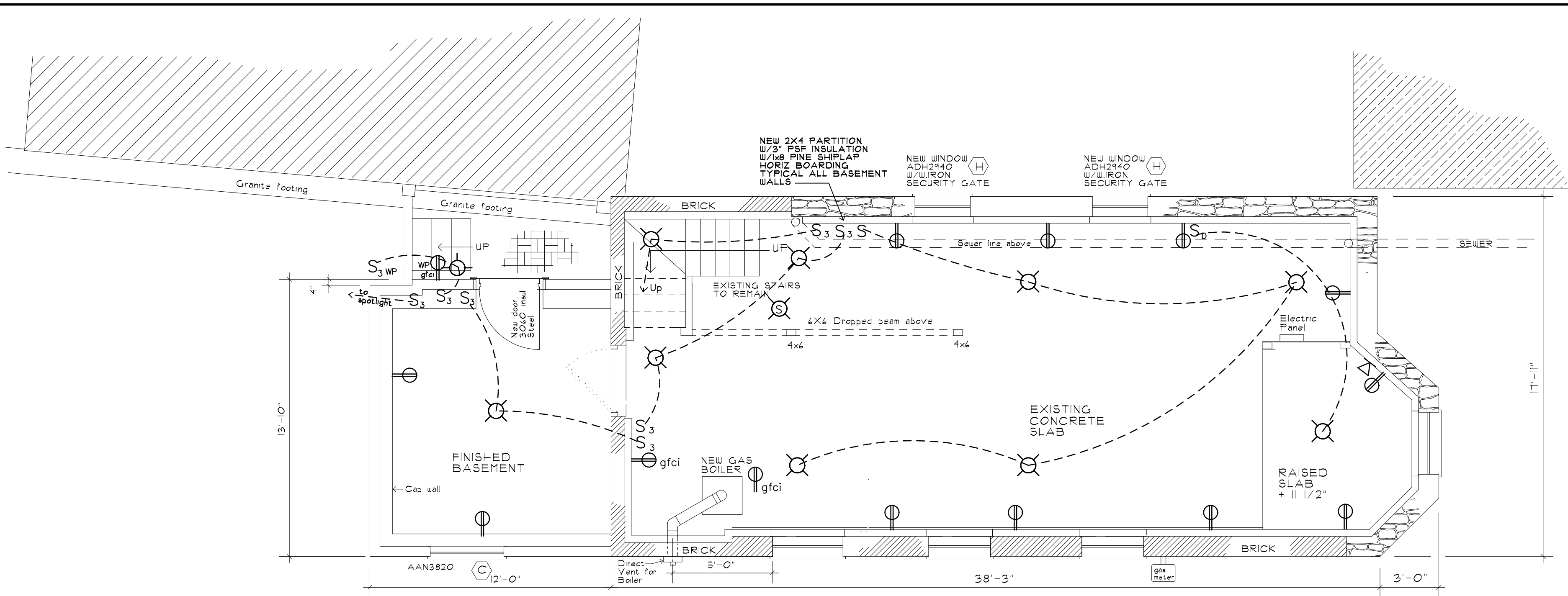
Remodeled Basement Electrical Plan 1/4"=1'-0"
