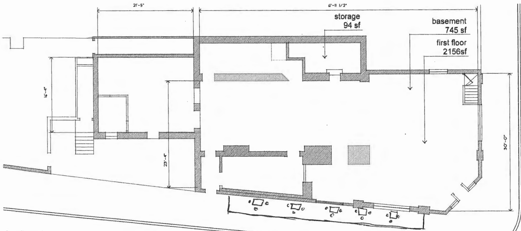
first floor plan approximate dimensions
