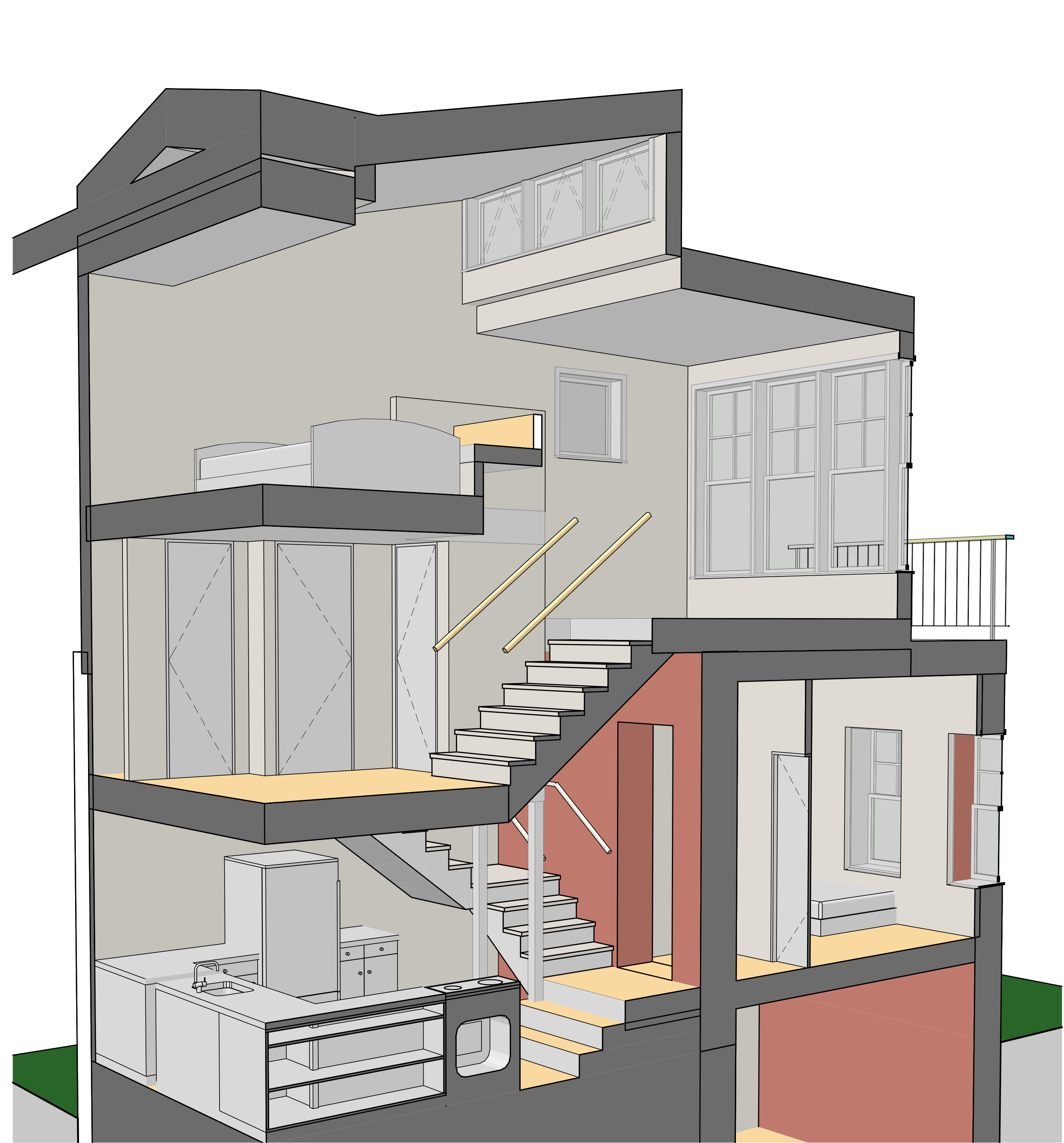
2 PERSPECTIVE CUTAWAY SCALE: 1:39.91
