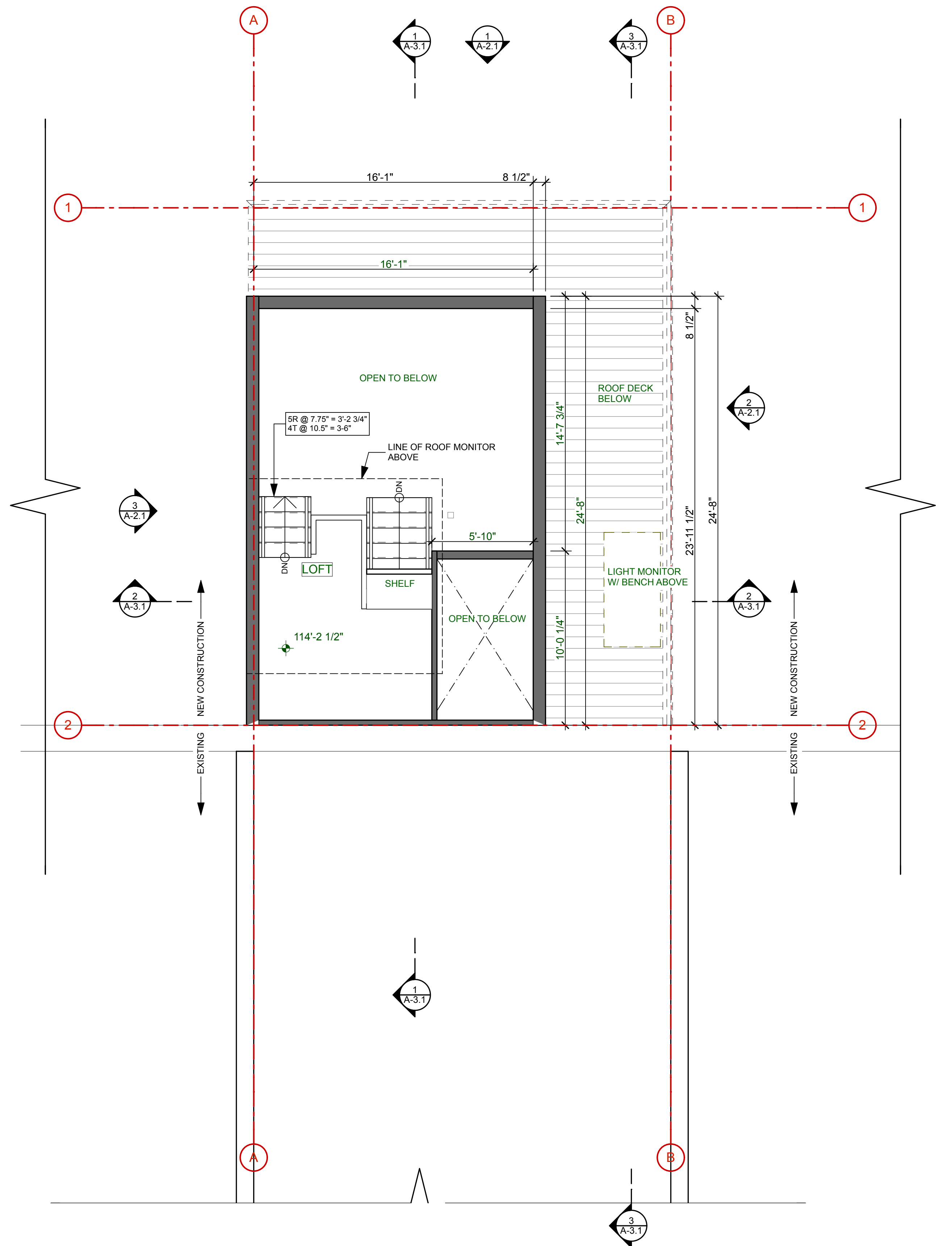
1 3rd FLOOR SCALE: 1/4" = 1'-0"
