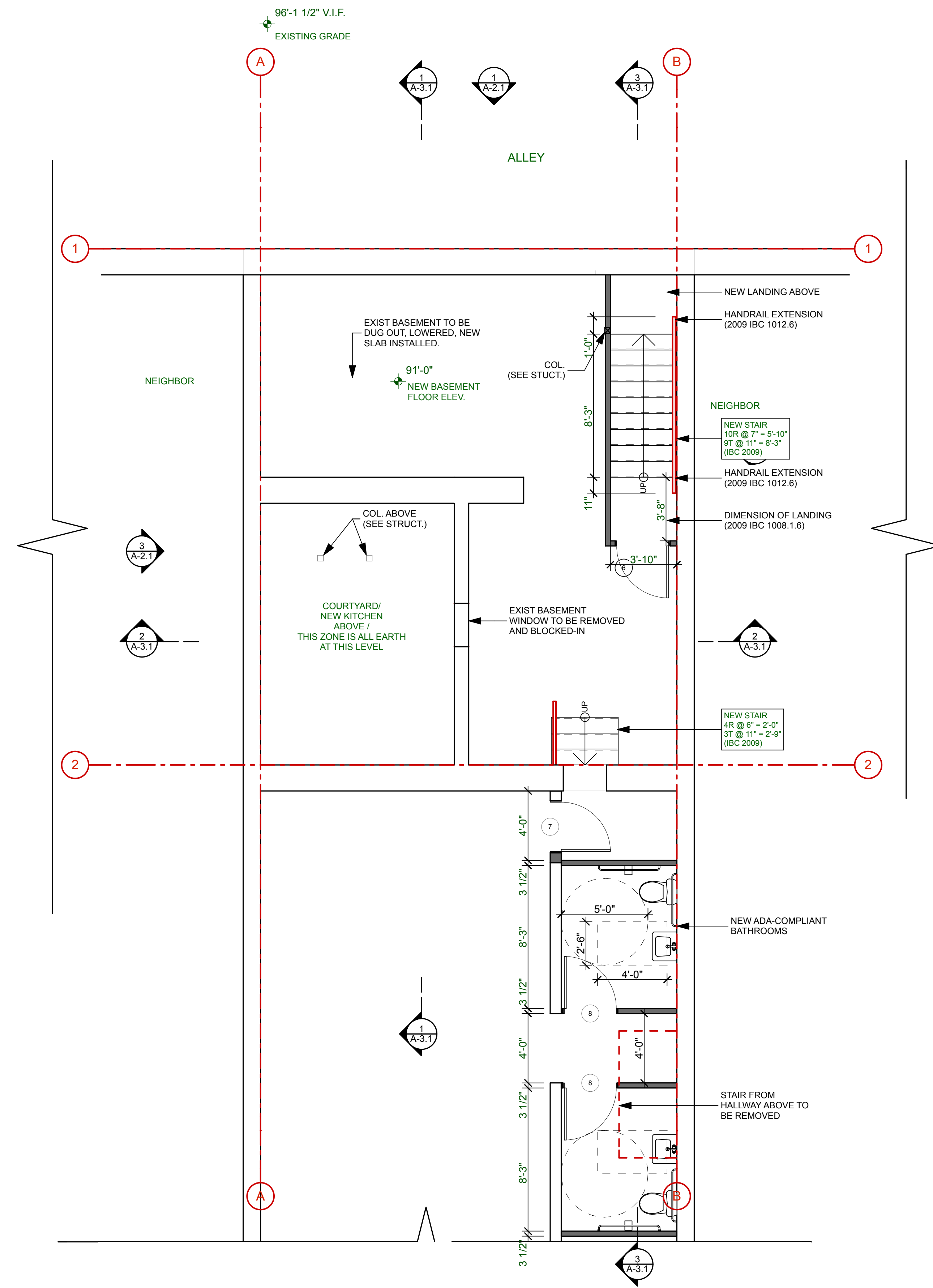
1 BASEMENT SCALE: 1/4" = 1'-0"
