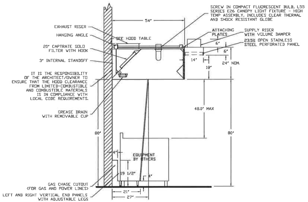
SECTION VIEW - MODEL 5424ND-2-PSP-FS HOOD - #1
