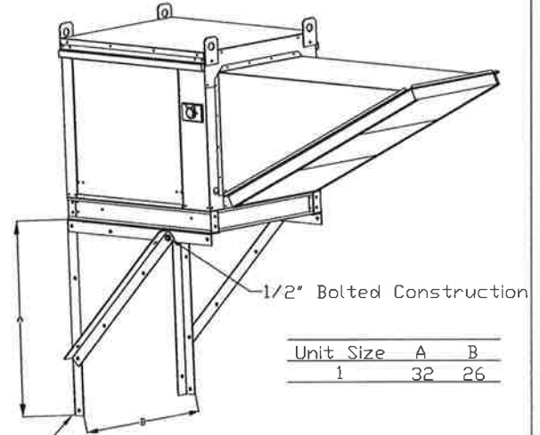
Untempered Supply Fan Wall Mount Bracket Detail
