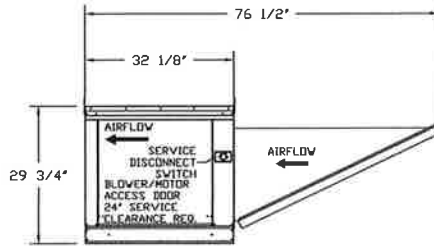
Untempered Supply Fan Wall Mount Bracket Detail
