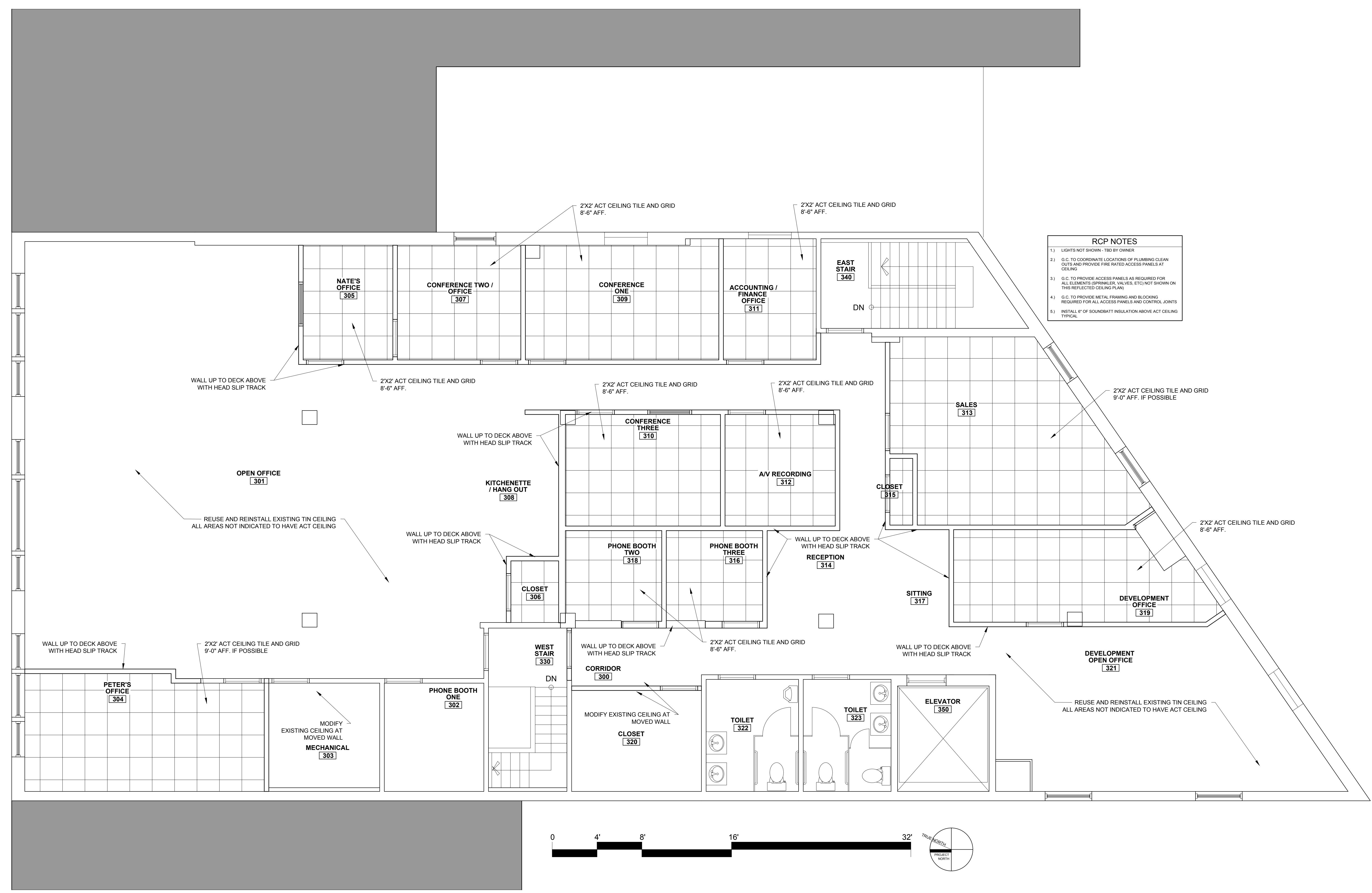
1 THIRD FLOOR REFLECTED CEILING PLAN 1/4" = 1'-0"
