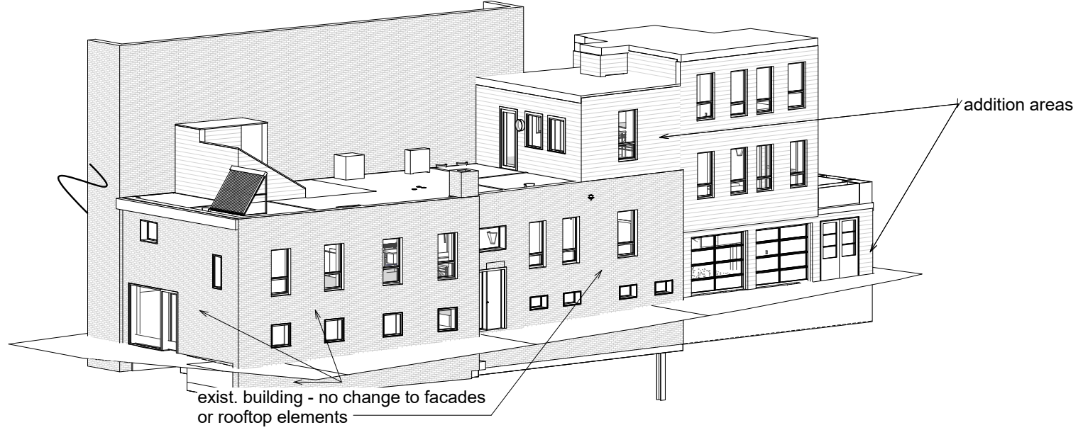
2 3D aerial view from south-east corner
