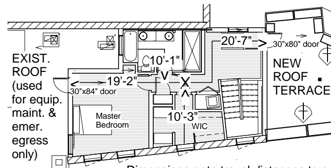
② Level 3 Egress Plan 1/8" = 1'-0"
