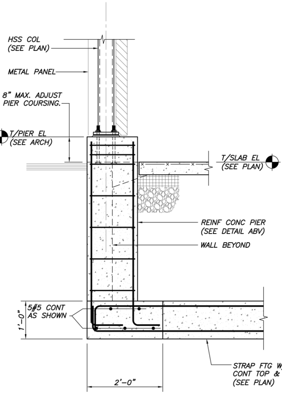
SECTION 3 3/4"=1'-0"
