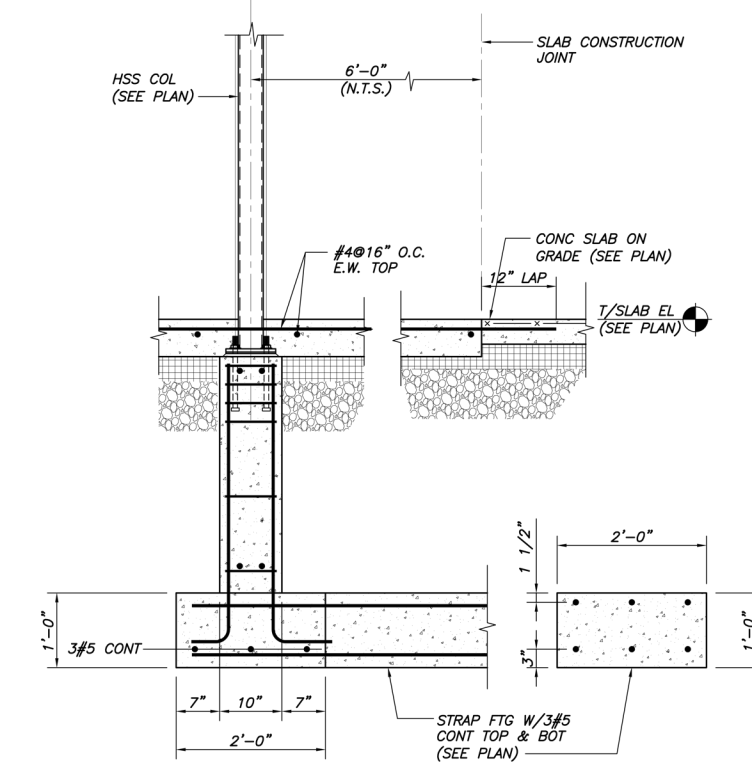
SECTION 1 3/4"=1'-0"
