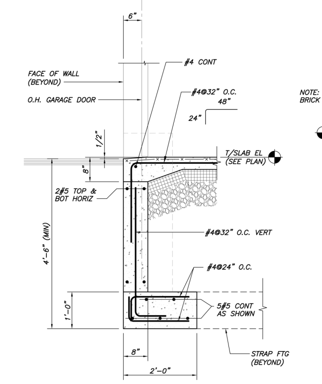
SECTION 2 3/4"=1'-0"
