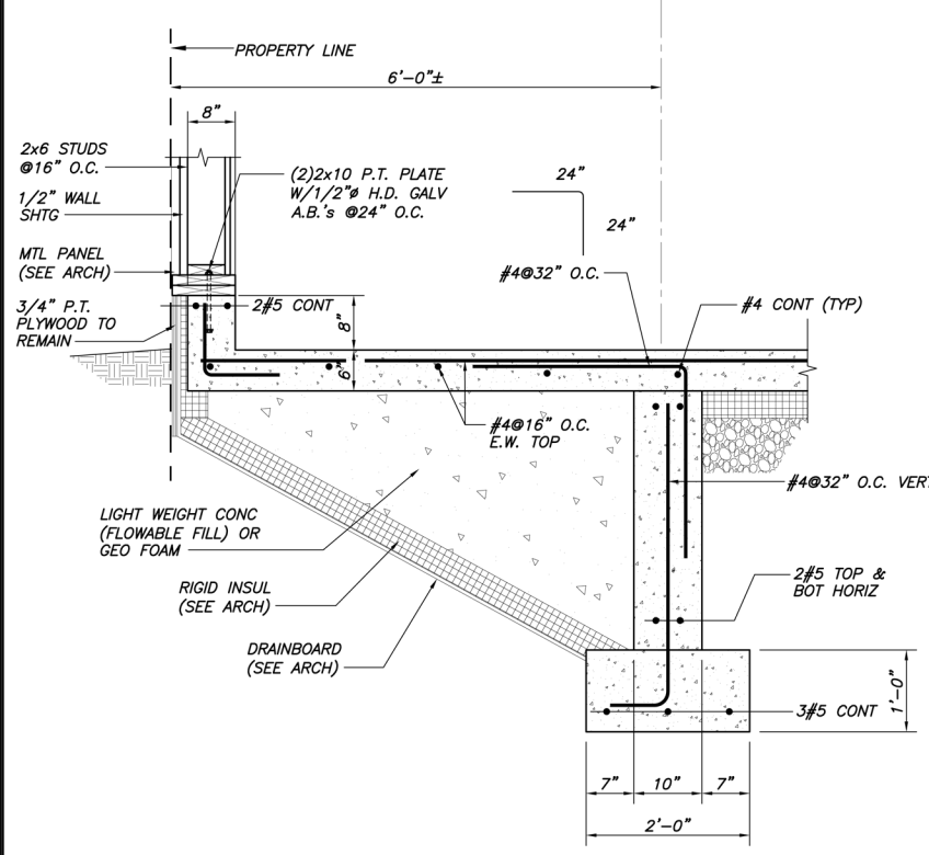
SECTION 1 3/4"=1'-0"
