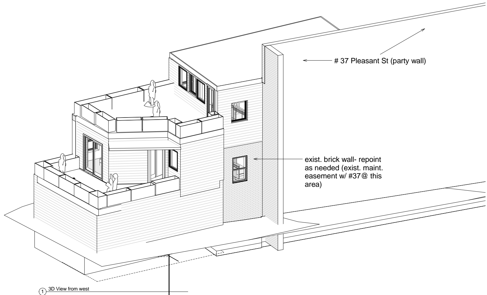
① 3D View from west
