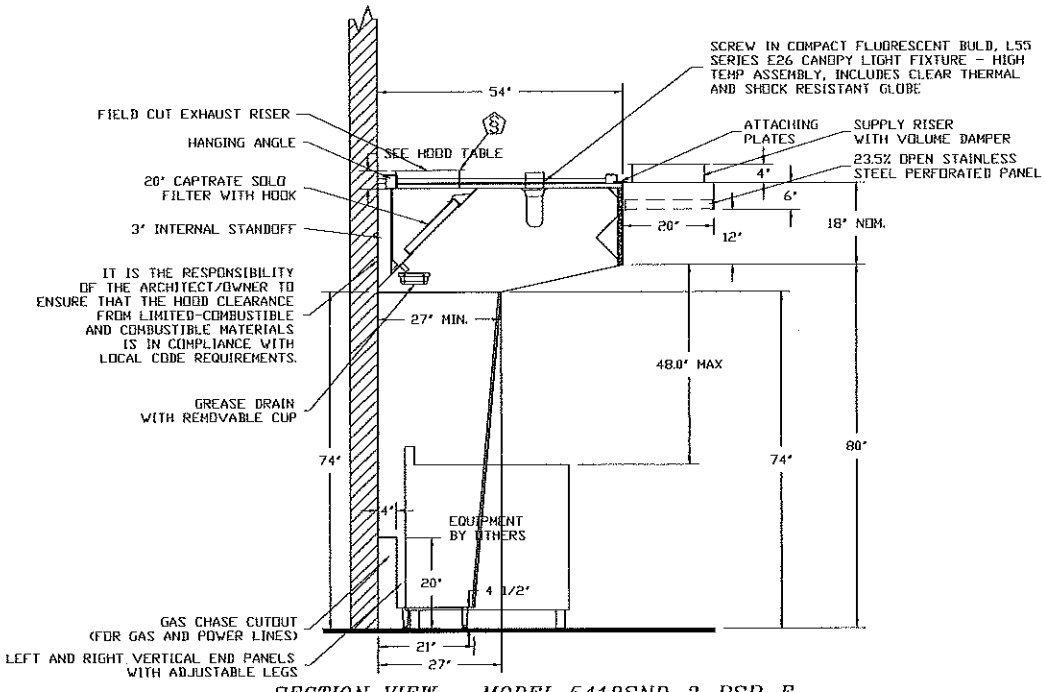
SECTION VIEW - MODEL 5418SND-2-PSP-F HOOD - #1
