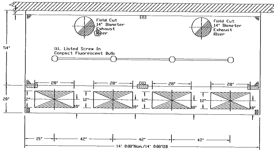
PLAN VIEW - Hood #1 14' 0.00" LONG 5418SND-2-PSP-F NOTE: Additional hanging angles provided for hoods 12' and longer.
