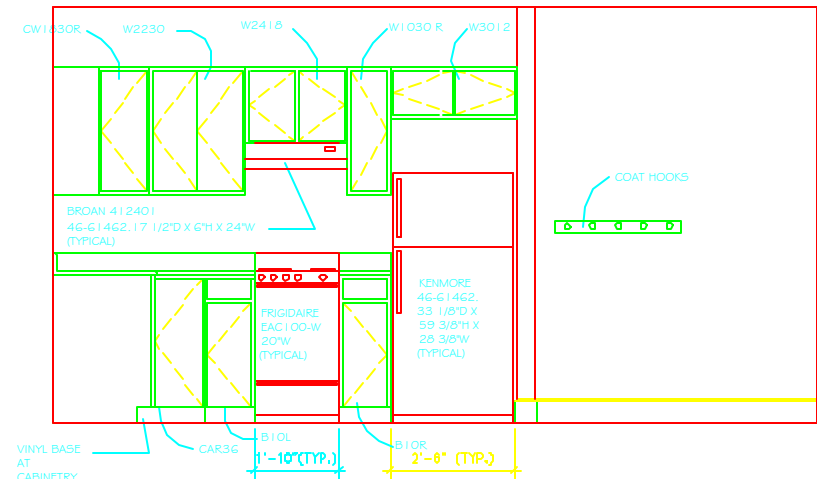
KITCHEN ELEV.
