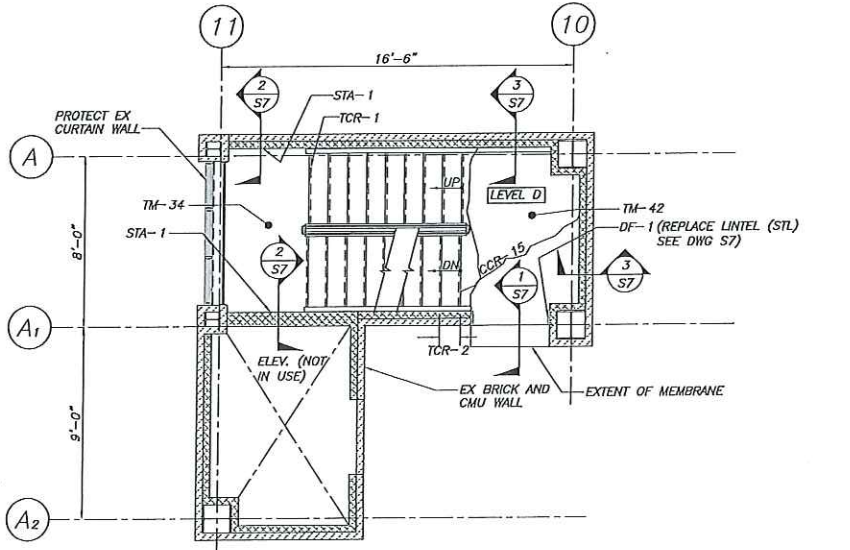
LEVEL D PLAN AT STAIR TOWER #1 1/4"=1'-0"
