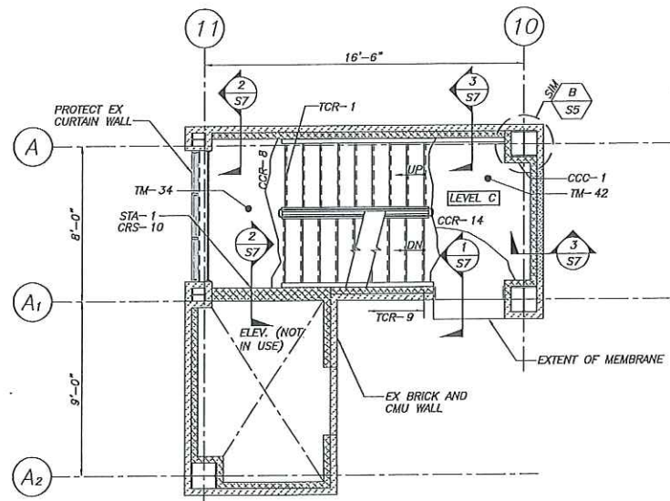
LEVEL C PLAN AT STAIR TOWER #1 1/4"=1'-0"
