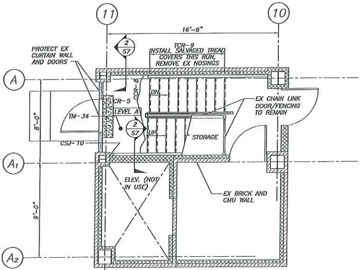
LEVEL A PLAN AT STAIR TOWER #1 1/4"=1'-0"
