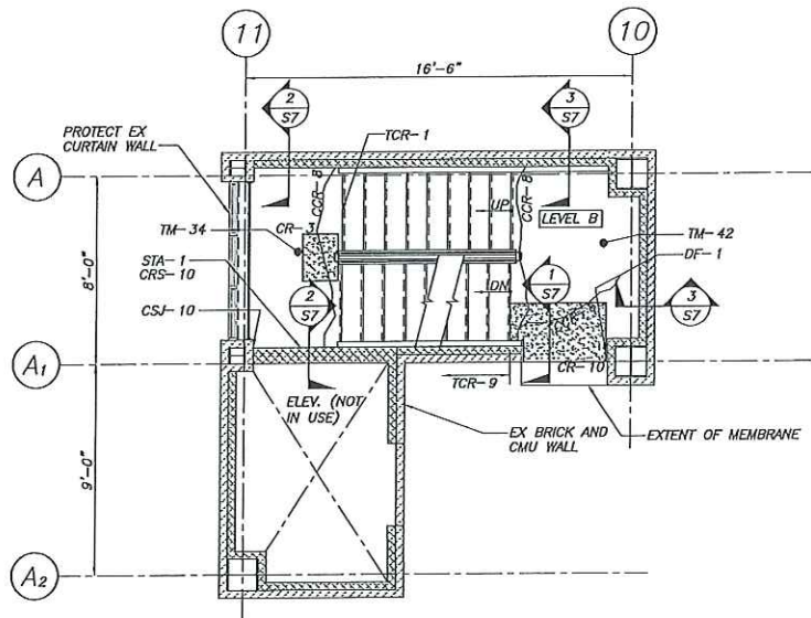
LEVEL B PLAN AT STAIR TOWER #1 1/4"=1'-0"
