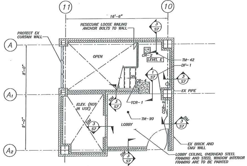
LEVEL E PLAN AT STAIR TOWER #1 1/4"=1'-0"
